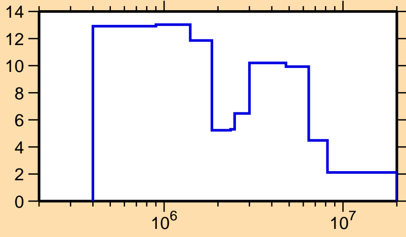
\Delta\sigma/\sigma vs. E for ^{161}\text{Tm}(n, tot.)
