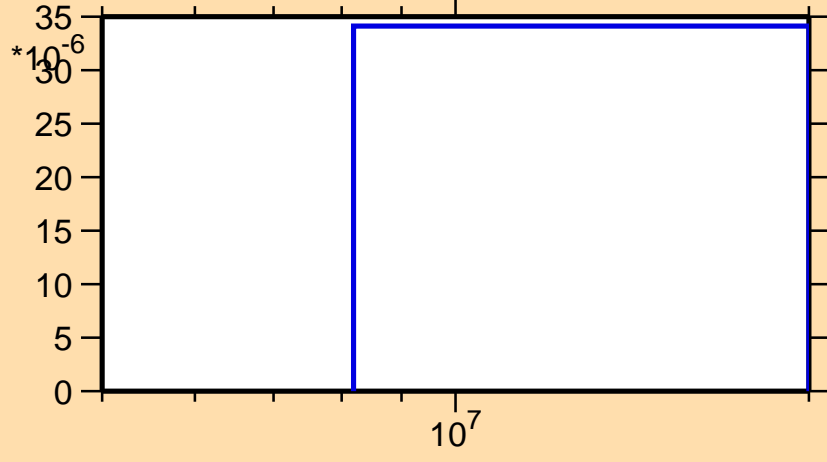
\sigma vs. E for ^{161}\text{Tm}(n,3n)
