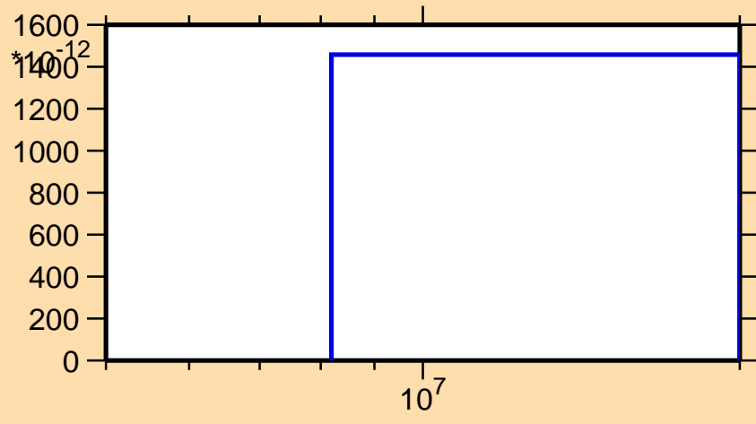
\sigma vs. E for ^{161}\text{Tm}(n,nt)
