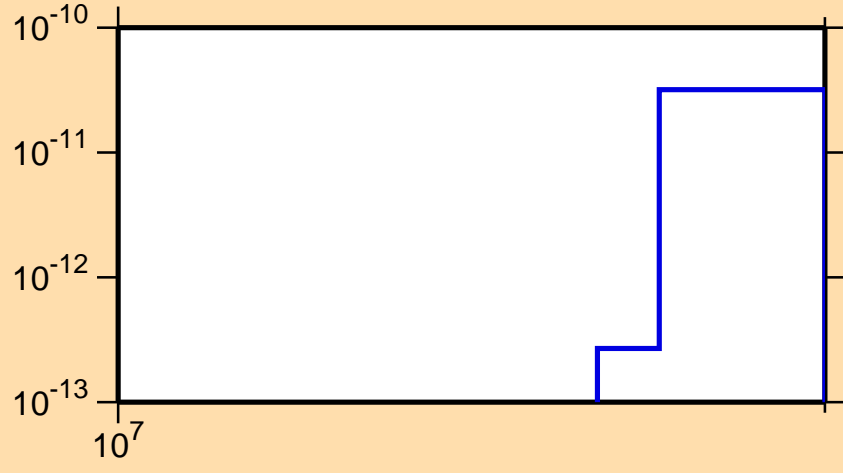
\sigma vs. E for ^{162}\text{Tm}(n,pt)
