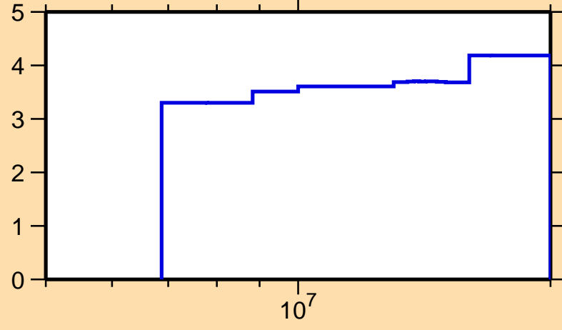
\Delta\sigma/\sigma vs. E for ^{162}\text{Tm}(n,\text{nonel.})
