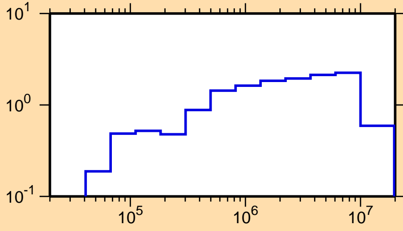
\sigma vs. E for ^{162}\text{Tm}(n,\text{inel.})
