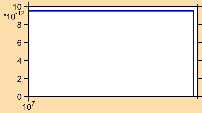
\sigma vs. E for ^{162}\text{Tm} (mt117)
