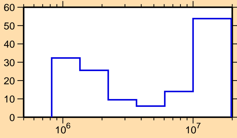
\Delta\sigma/\sigma vs. E for ^{162}\text{Tm}(n,ncont.)
