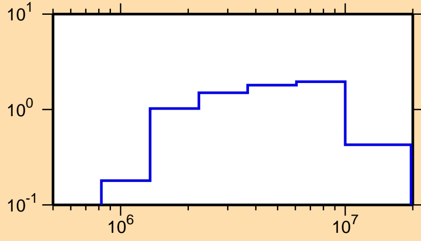
\sigma vs. E for ^{162}\text{Tm}(n,n\text{cont.})
