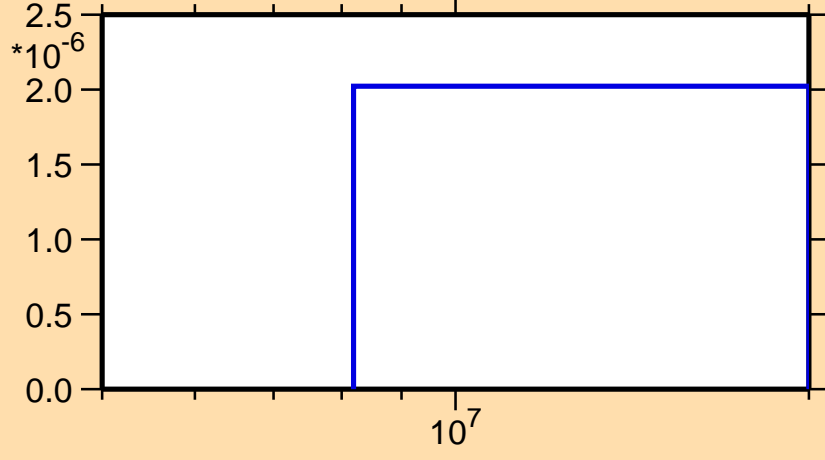
\sigma vs. E for ^{162}\text{Tm}(n,\text{nd})
