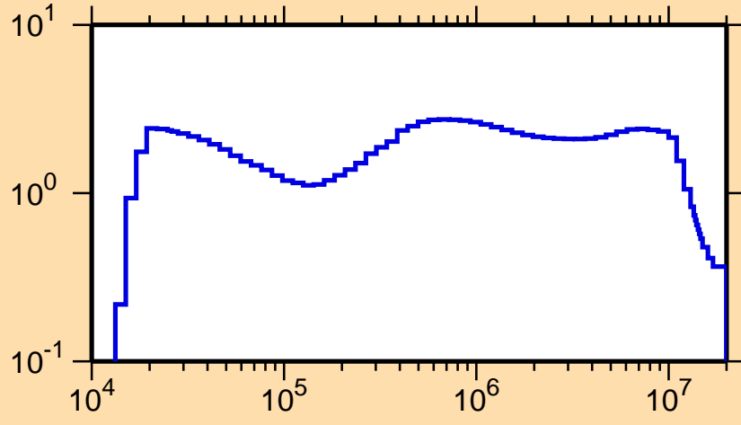
\sigma vs. E for ^{163}\text{Tm}(n,\text{inel.})
