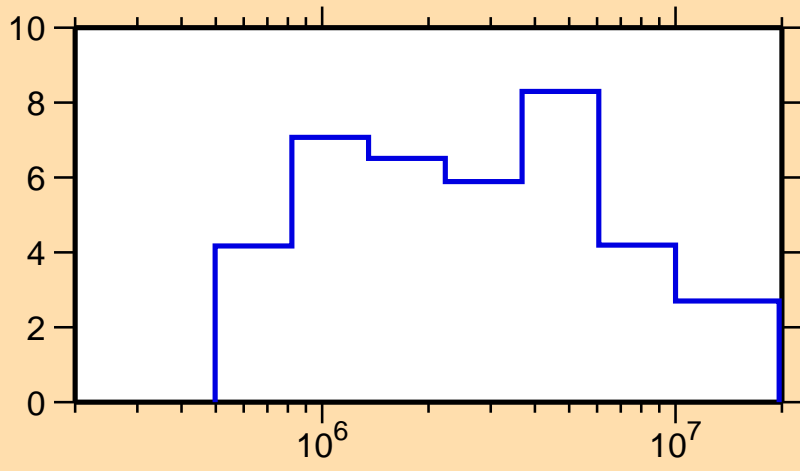
\Delta\sigma/\sigma vs. E for ^{163}\text{Tm}(n, el.)
