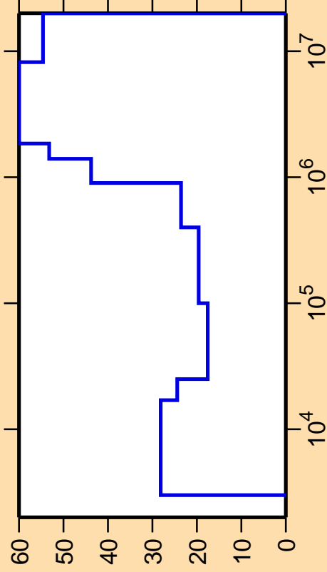
\Delta\sigma/\sigma vs. E for ^{163}\text{Tm}(n,\gamma)
