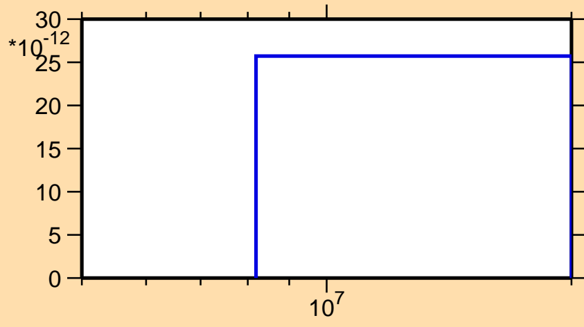
\sigma vs. E for ^{163}\text{Tm} (mt 45)
