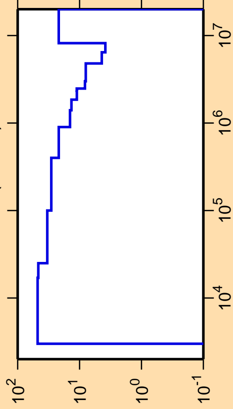
\Delta\sigma/\sigma vs. E for ^{163}\text{Tm}(n,\text{inel.})
