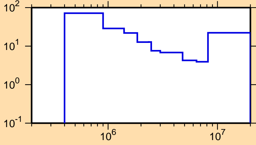
\Delta\sigma/\sigma vs. E for ^{163}\text{Tm}(n,n\text{cont.})
