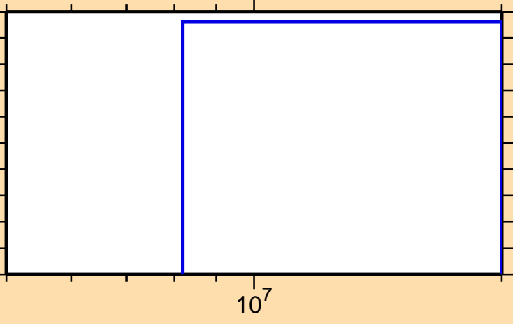
\sigma vs. E for ^{163}\text{Tm}(n,nt)
