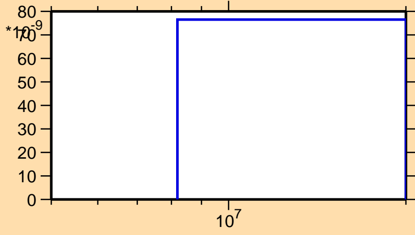
\sigma vs. E for ^{163}\text{Tm}(n,\text{nd})
