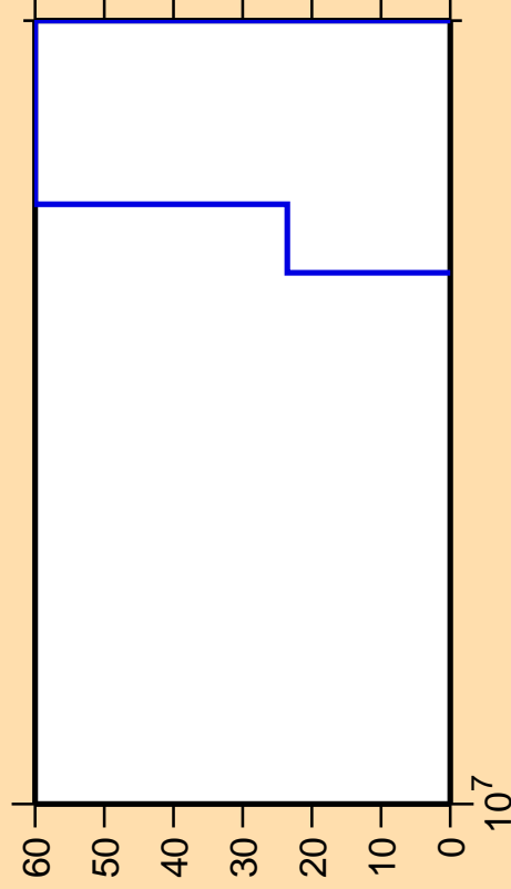
\Delta\sigma/\sigma vs. E for ^{164}\text{Tm} (mt117)
