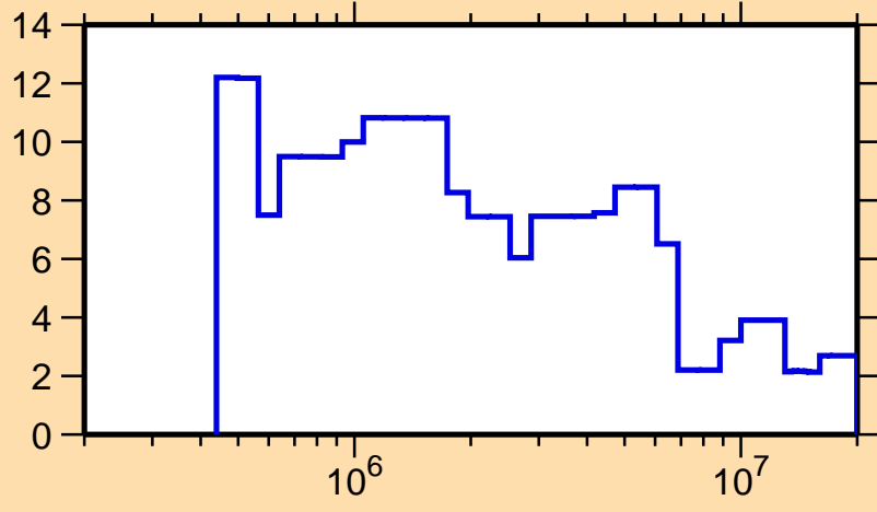
\Delta\sigma/\sigma vs. E for ^{164}\text{Tm}(n, el.)
