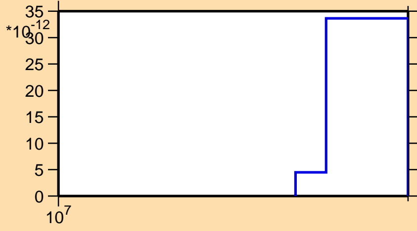
\sigma vs. E for ^{164}\text{Tm} (mt117)
