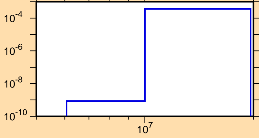
\sigma vs. E for ^{164}\text{Tm}(n,t)
