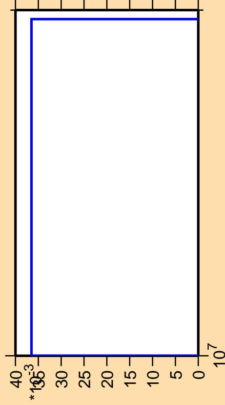
\Delta\sigma/\sigma vs. E for ^{166}\text{Tm} (mt 45)
