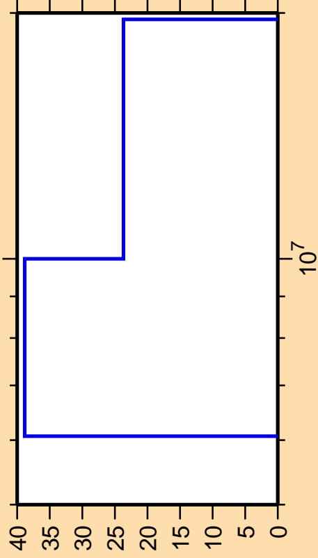
\Delta\sigma/\sigma vs. E for ^{166}\text{Tm}(n,np)
