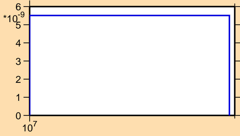
\sigma vs. E for ^{166}\text{Tm}(n,nt)
