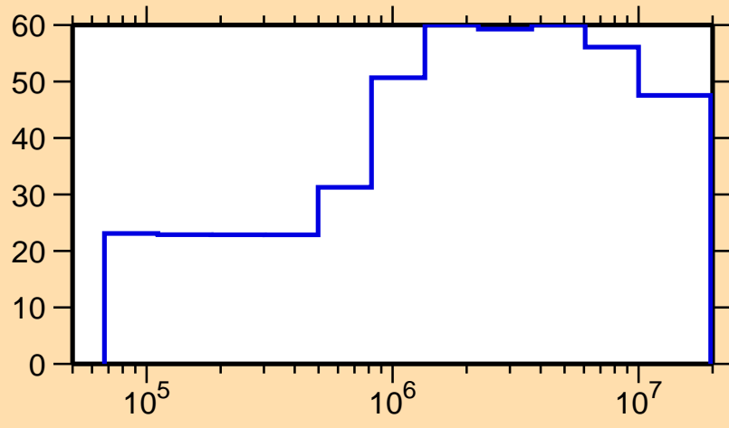
\Delta\sigma/\sigma vs. E for ^{166}\text{Tm}(n,n_1)
