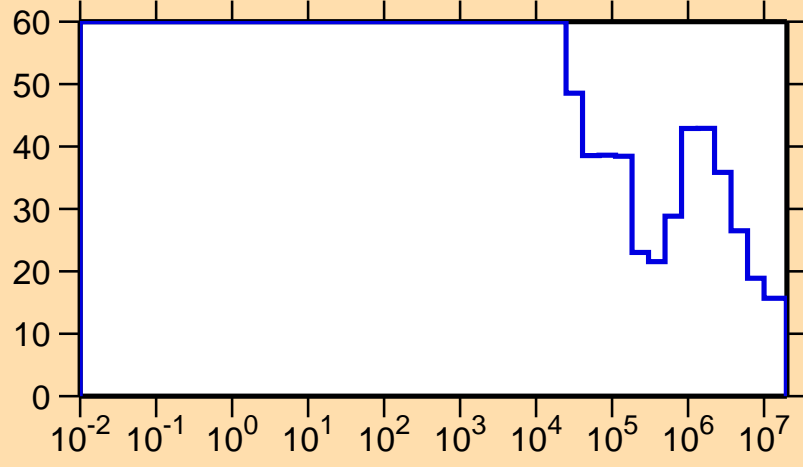
\Delta\sigma/\sigma vs. E for ^{166}\text{Tm}(n,p)
