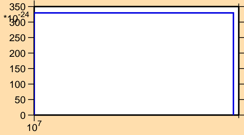
\sigma vs. E for ^{166}\text{Tm} (mt 11)
