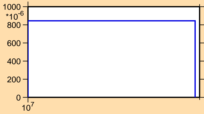
\sigma vs. E for ^{166}\text{Tm}(n,3n)
