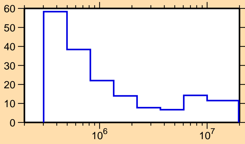
\Delta\sigma/\sigma vs. E for ^{166}\text{Tm}(n,ncont.)
