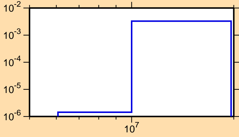
\sigma vs. E for ^{166}\text{Tm}(n,np)
