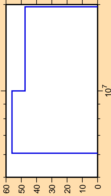
\Delta\sigma/\sigma vs. E for ^{166}\text{Tm}(n,n_1)
