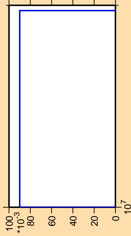
\Delta\sigma/\sigma vs. E for ^{166}\text{Tm}(\text{mt117})
