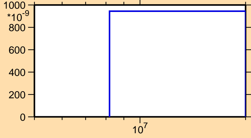
\sigma vs. E for ^{166}\text{Tm}(n,nd)
