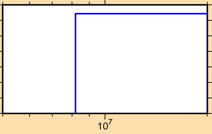
\sigma vs. E for ^{166}\text{Tm}(n,\text{He}3)
