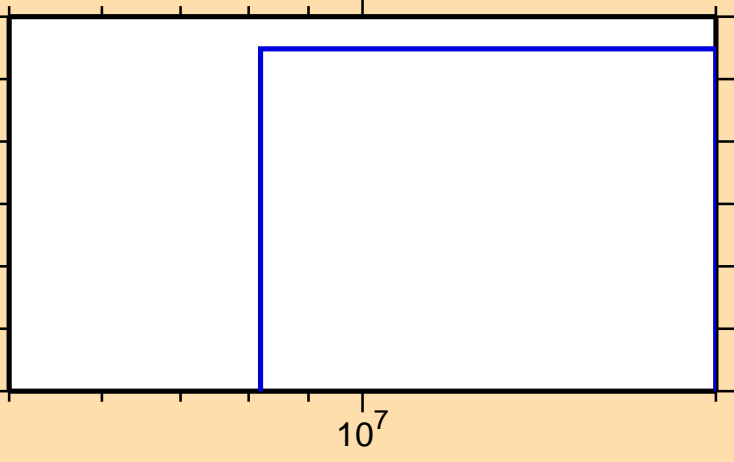
\sigma vs. E for ^{166}\text{Tm}(n,nt)
