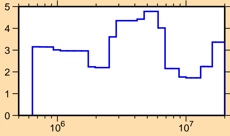
\Delta\sigma/\sigma vs. E for ^{167}\text{Tm}(n,el.)
