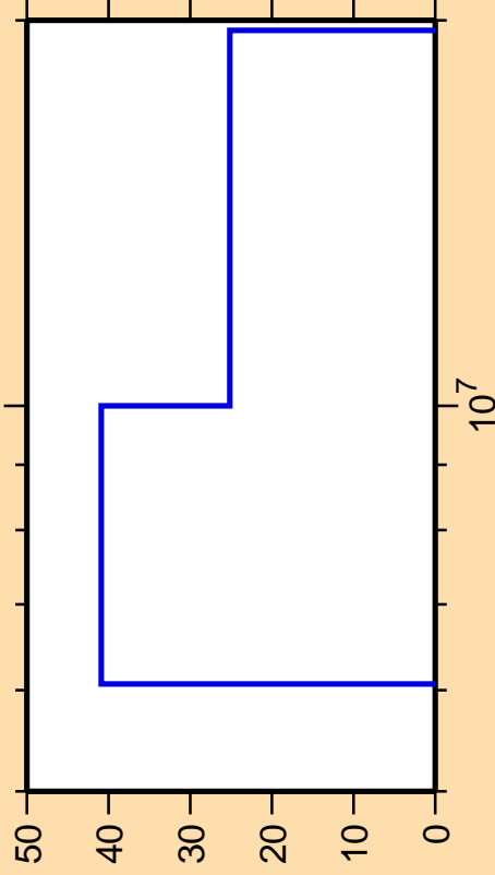
\Delta\sigma/\sigma vs. E for ^{167}\text{Tm}(n,\gamma)
