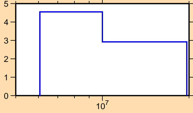
\Delta\sigma/\sigma vs. E for ^{167}\text{Tm}(n,2n)
