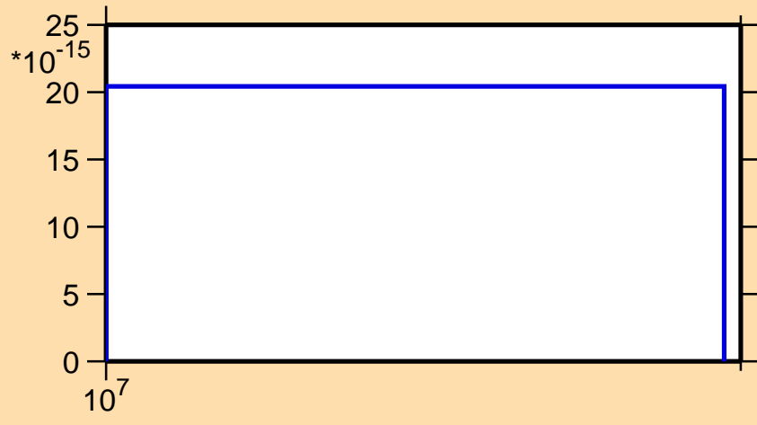
\sigma vs. E for ^{167}\text{Tm}(\text{mt117})
