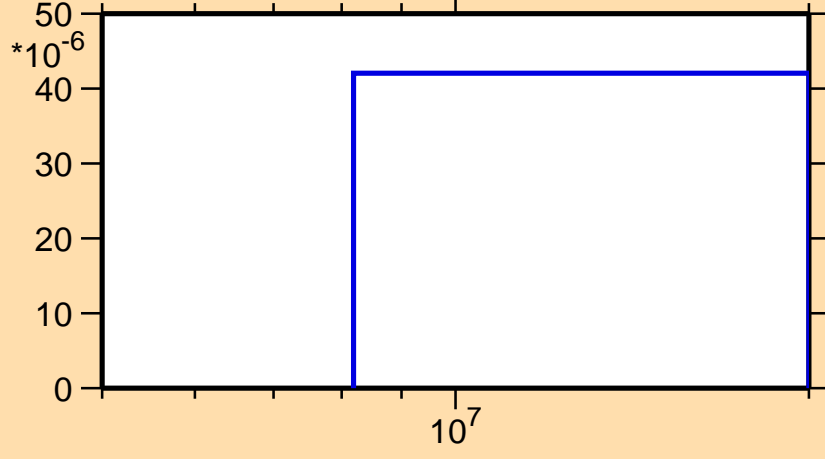
\sigma vs. E for ^{167}\text{Tm}(n,t)
