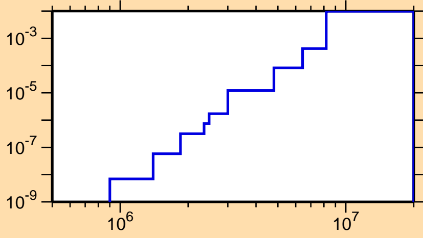
\sigma vs. E for ^{167}\text{Tm}(n,p)
