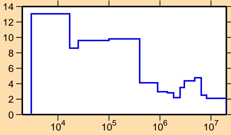
\Delta\sigma/\sigma vs. E for ^{167}\text{Tm}(n,\text{el.})
