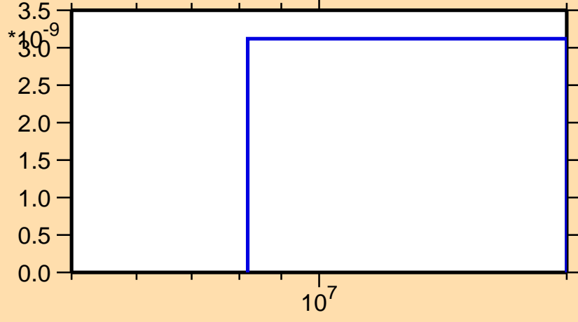
\sigma vs. E for ^{167}\text{Tm}(n,nt)
