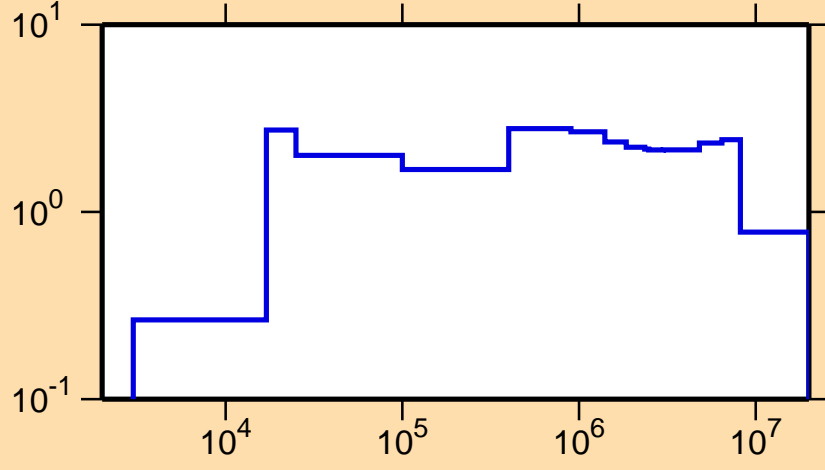
\sigma vs. E for ^{167}\text{Tm}(n,\text{inel.})
