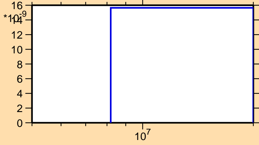
\sigma vs. E for ^{167}\text{Tm}(n,2np)
