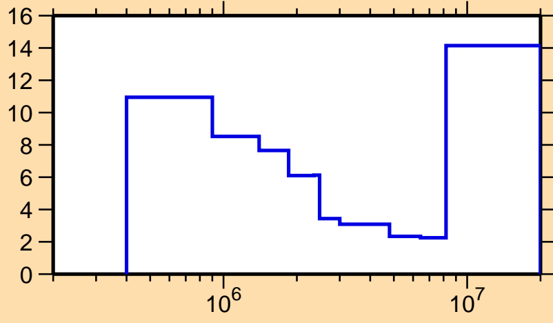
\Delta\sigma/\sigma vs. E for ^{167}\text{Tm}(n,\text{inel.})
