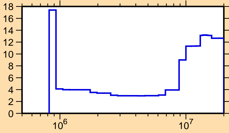
\Delta\sigma/\sigma vs. E for ^{169}\text{Tm}(n,ncont.)
