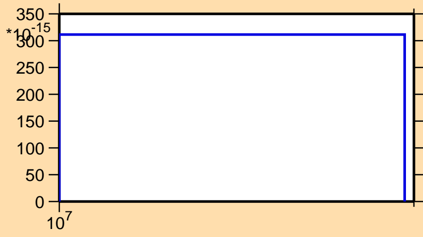
\sigma vs. E for ^{169}\text{Tm}(n,p\alpha)
