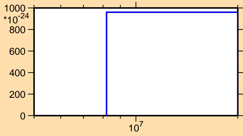
\sigma vs. E for ^{169}\text{Tm} (mt 42)
