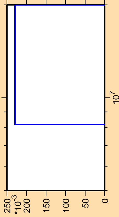
\Delta\sigma/\sigma vs. E for ^{169}\text{Tm}(n,p\alpha)
