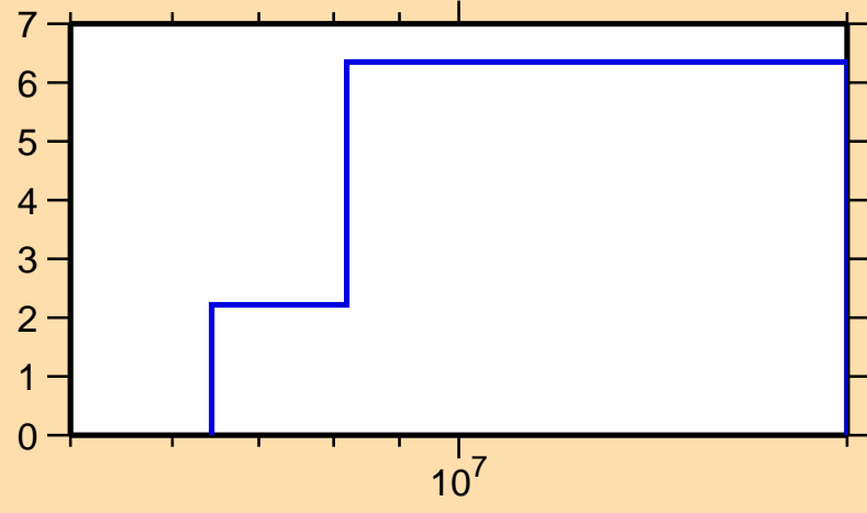
\Delta\sigma/\sigma vs. E for ^{169}\text{Tm}(n,\text{inel.})
