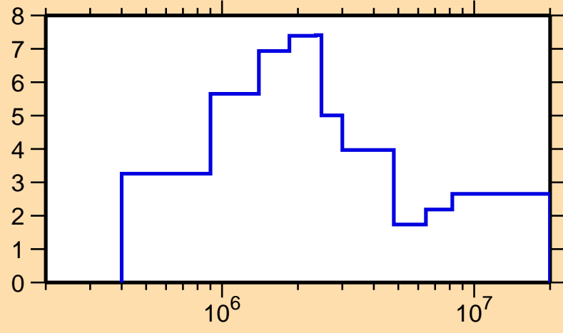
\Delta\sigma/\sigma vs. E for ^{169}\text{Tm}(n, el.)
