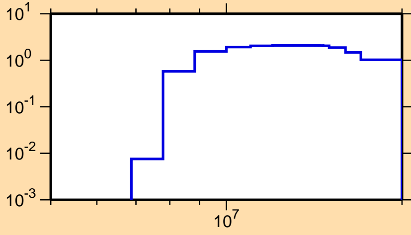
\sigma vs. E for ^{171}\text{Tm}(n,2n)
