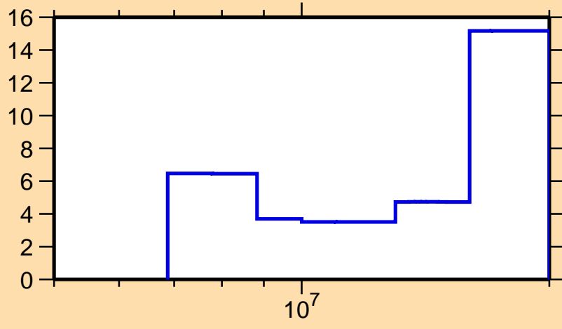
\Delta\sigma/\sigma vs. E for ^{171}\text{Tm}(n,2n)
