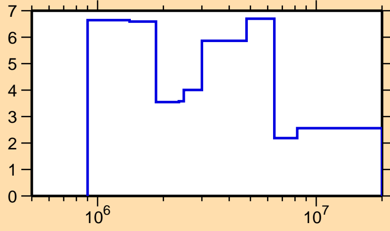
\Delta\sigma/\sigma vs. E for ^{171}\text{Tm}(n, el.)
