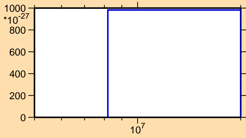
\sigma vs. E for ^{171}\text{Tm} (mt 42)
