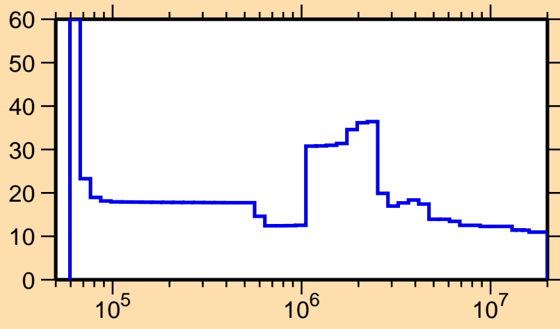
\Delta\sigma/\sigma vs. E for ^{172}\text{Tm}(n,n_1)
