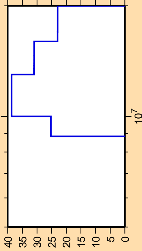
\Delta\sigma/\sigma vs. E for ^{172}\text{Tm}(n,np)
