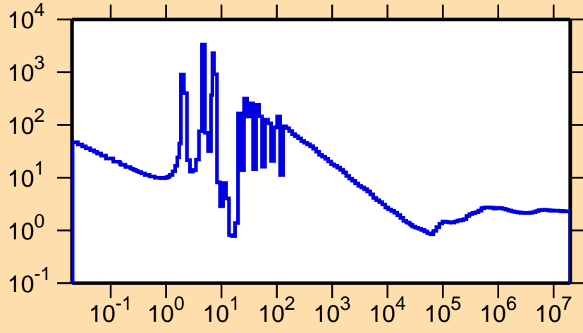
\sigma vs. E for ^{172}\text{Tm}(n,\text{nonel.})
