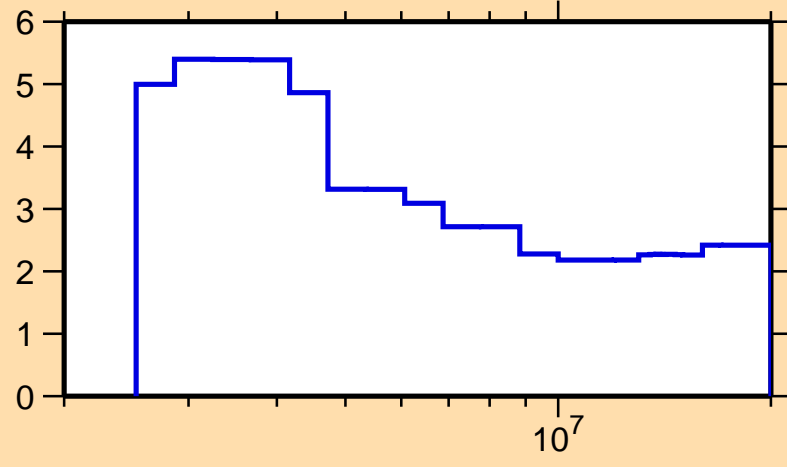
\Delta\sigma/\sigma vs. E for ^{172}\text{Tm}(n,\text{nonel.})
