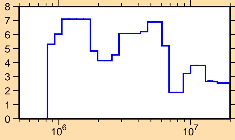
\Delta\sigma/\sigma vs. E for ^{172}\text{Tm}(n, \text{el.})
