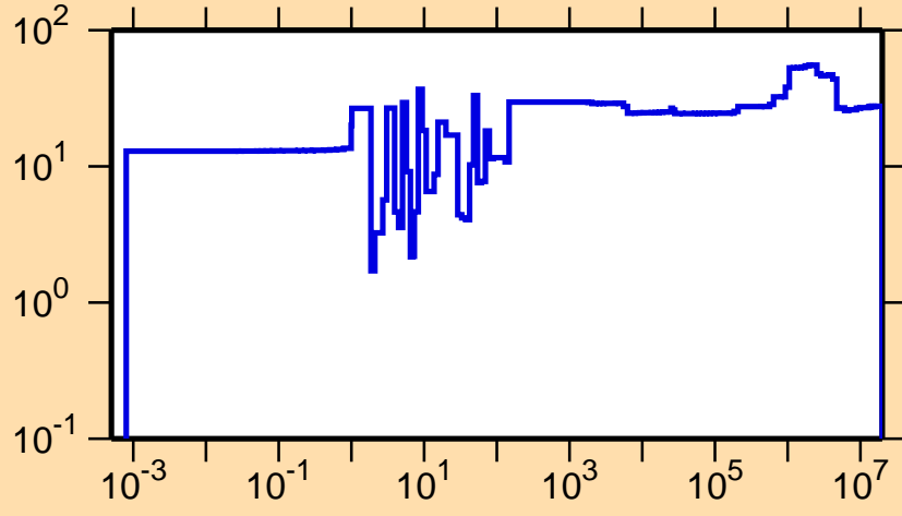
\Delta\sigma/\sigma vs. E for ^{172}\text{Tm}(n,\gamma)
