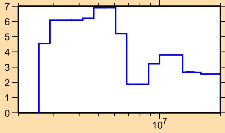
\Delta\sigma/\sigma vs. E for ^{172}\text{Tm}(n,el.)
