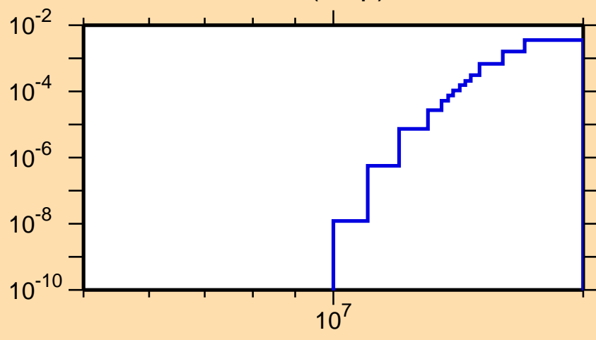
\sigma vs. E for ^{172}\text{Tm}(n,np)
