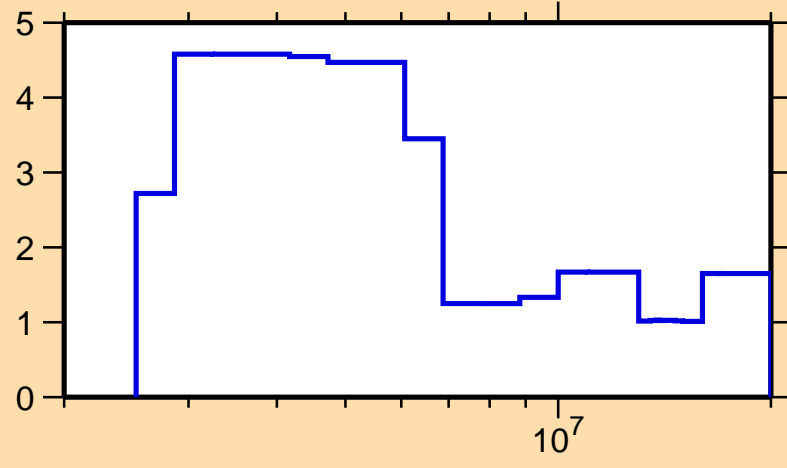
\Delta\sigma/\sigma vs. E for ^{172}\text{Tm}(n,\text{tot.})
