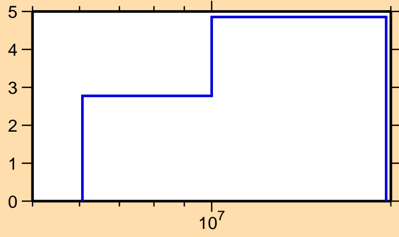
\Delta\sigma/\sigma vs. E for ^{172}\text{Tm}(n,2n)
