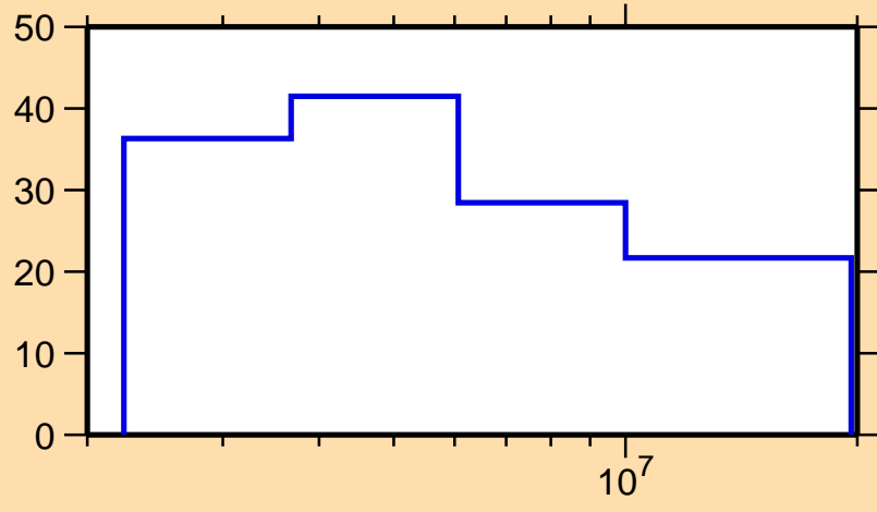
\Delta\sigma/\sigma vs. E for ^{172}\text{Tm}(n,p)
