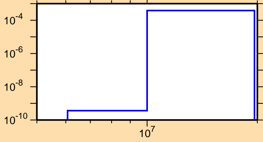
\sigma vs. E for ^{172}\text{Tm}(n,d)
