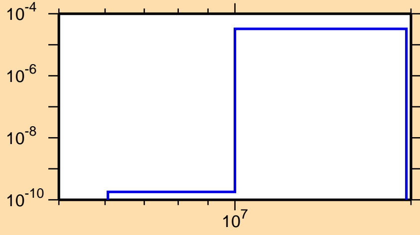
\sigma vs. E for ^{172}\text{Tm}(n,n\alpha)
