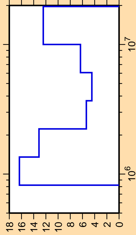
\Delta\sigma/\sigma vs. E for ^{172}\text{Tm}(n,ncont.)
