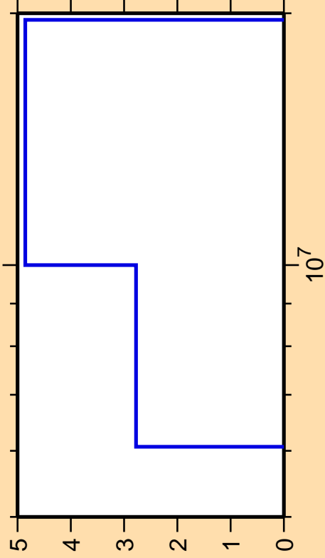
\Delta\sigma/\sigma vs. E for ^{172}\text{Tm}(n,2n)
