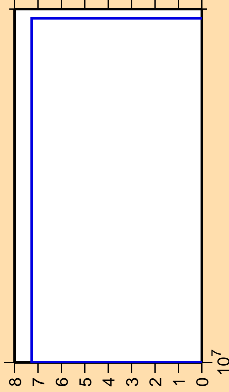
\Delta\sigma/\sigma vs. E for ^{172}\text{Tm}(n,3n)
