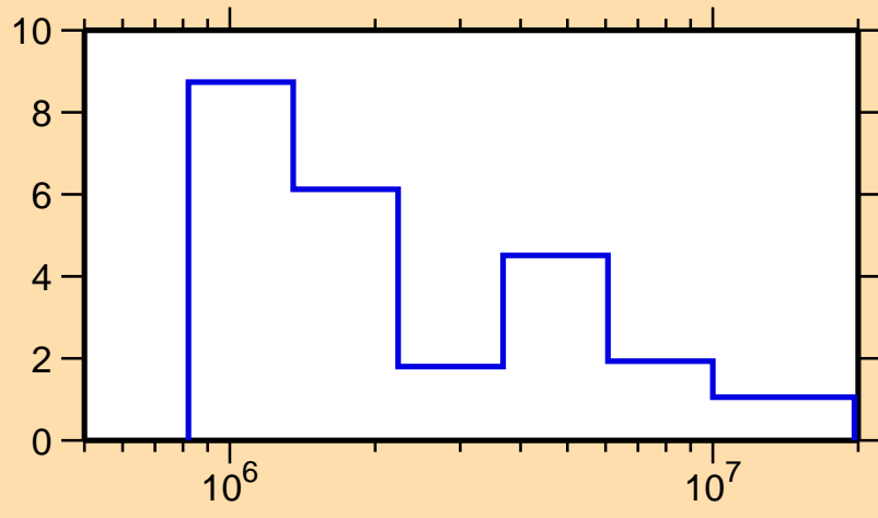
\Delta\sigma/\sigma vs. E for ^{172}\text{Tm}(n, tot.)
