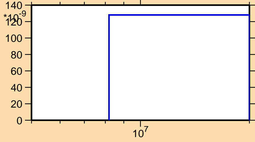
\sigma vs. E for ^{172}\text{Tm}(n,\text{nd})
