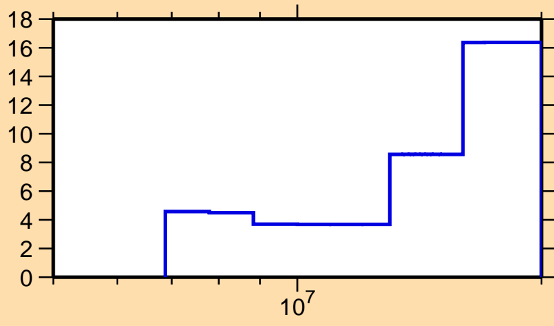
\Delta\sigma/\sigma vs. E for ^{173}\text{Tm}(n,2n)
