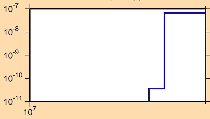
\sigma vs. E for ^{173}\text{Tm}(n,2np)
