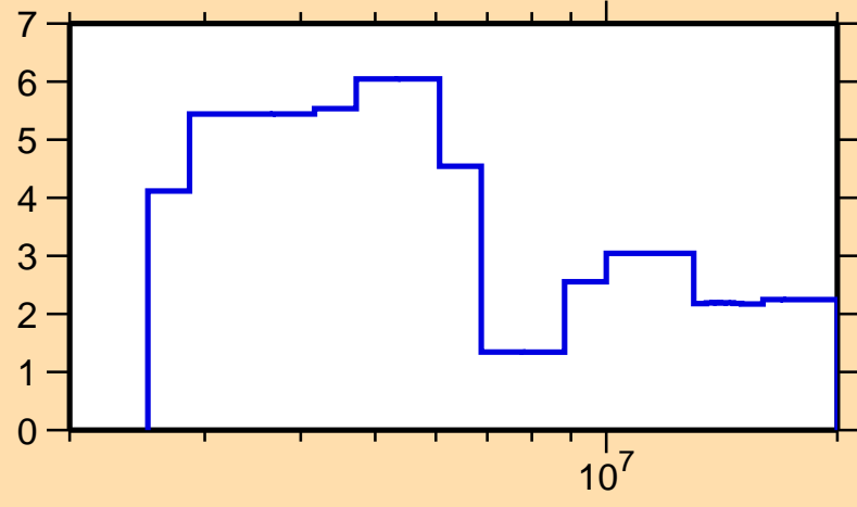
\Delta\sigma/\sigma vs. E for ^{173}\text{Tm}(n,el.)
