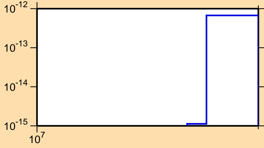
\sigma vs. E for ^{173}\text{Tm}(n,\text{He}3)
