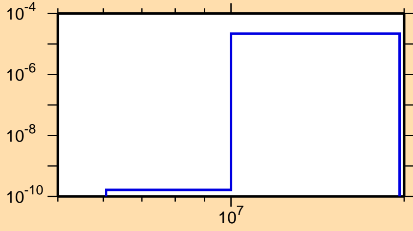
\sigma vs. E for ^{173}\text{Tm}(n,n\alpha)
