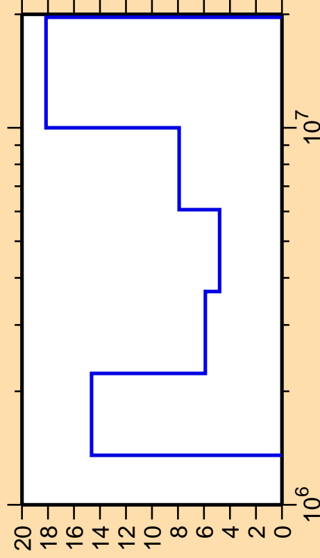
\Delta\sigma/\sigma vs. E for ^{173}\text{Tm}(n,ncont.)
