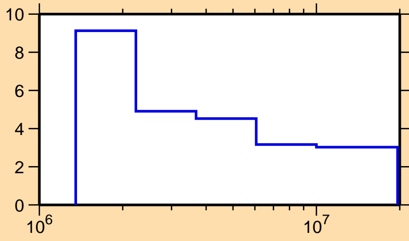
\Delta\sigma/\sigma vs. E for ^{173}\text{Tm}(n,nonel.)
