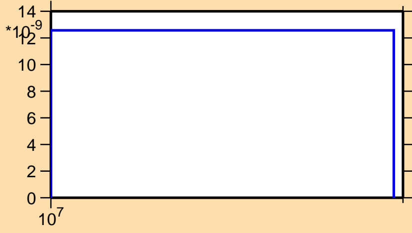
\sigma vs. E for ^{173}\text{Tm}(n,\text{nd})
