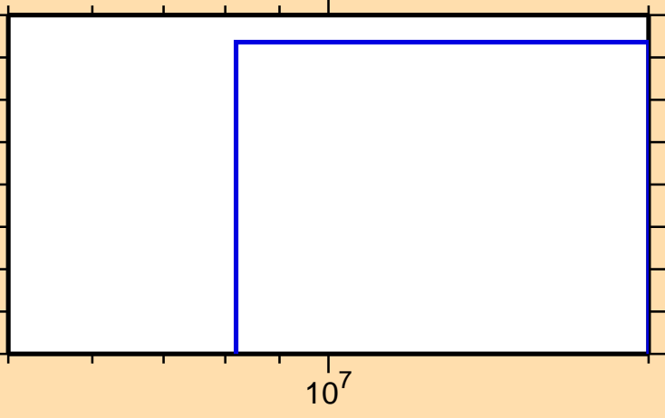
\sigma vs. E for ^{173}\text{Tm}(n,nt)
