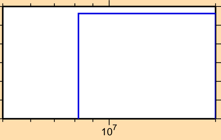
\sigma vs. E for ^{173}\text{Tm} (mt 42)
