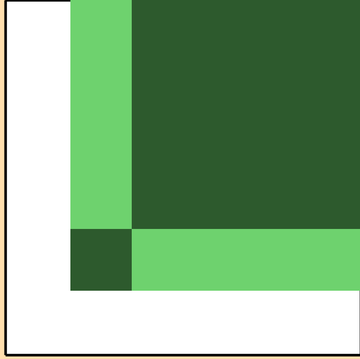
\sigma vs. E for ^{173}\text{Tm}(n,2n)
