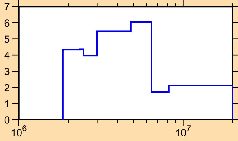
\Delta\sigma/\sigma vs. E for ^{173}\text{Tm}(n,\text{el.})
