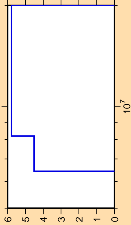
\Delta\sigma/\sigma vs. E for ^{173}\text{Tm}(n,2n)
