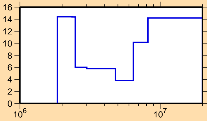
\Delta\sigma/\sigma vs. E for ^{173}\text{Tm}(n,n\text{cont.})
