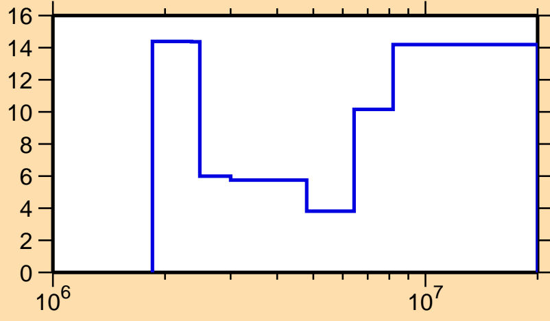
\Delta\sigma/\sigma vs. E for ^{173}\text{Tm}(n,ncont.)
