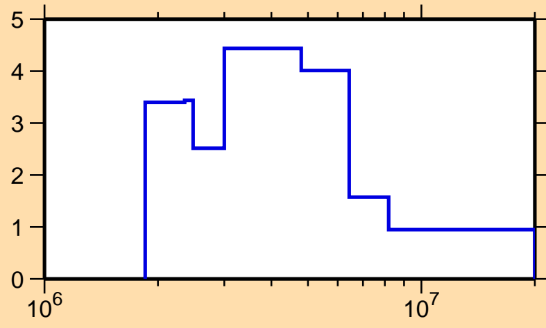
\Delta\sigma/\sigma vs. E for ^{173}\text{Tm}(n, tot.)
