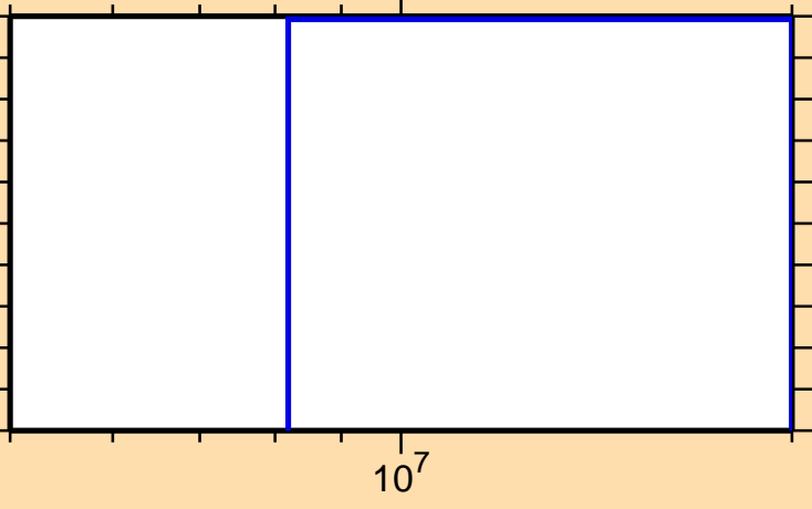
\sigma vs. E for ^{173}\text{Tm}(n,t)
