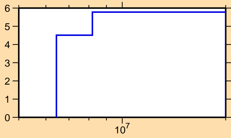
\Delta\sigma/\sigma vs. E for ^{173}\text{Tm}(n,2n)
