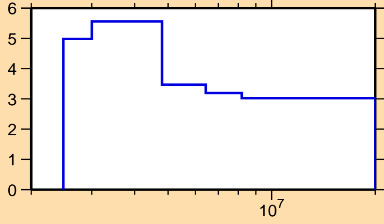
\Delta\sigma/\sigma vs. E for ^{173}\text{Tm}(n,\text{nonel.})
