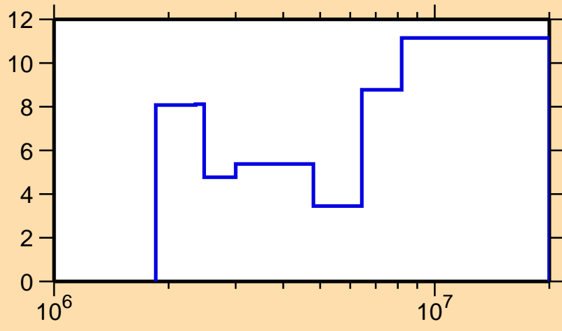
\Delta\sigma/\sigma vs. E for ^{173}\text{Tm}(n,\text{inel.})
