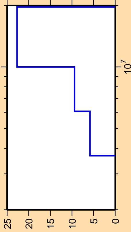
\Delta\sigma/\sigma vs. E for ^{174}\text{Tm}(n,n\text{cont.})
