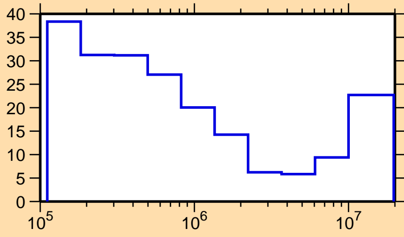
\Delta\sigma/\sigma vs. E for ^{174}\text{Tm}(n,ncont.)
