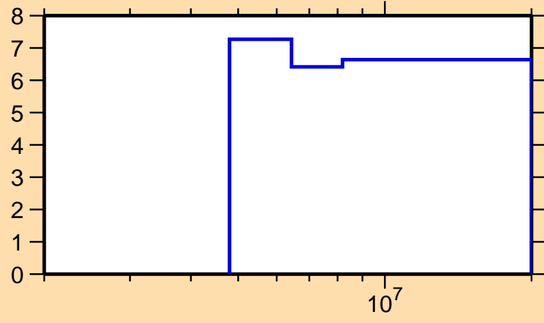
\Delta\sigma/\sigma vs. E for ^{174}\text{Tm}(n,2n)
