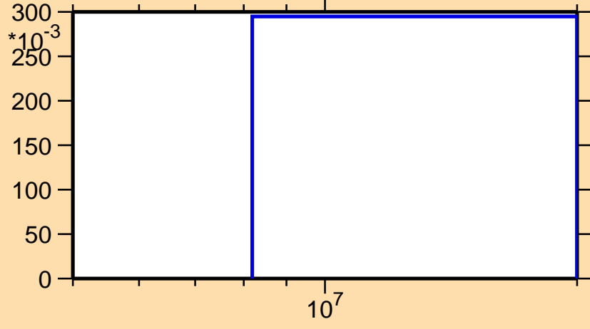
\sigma vs. E for ^{174}\text{Tm}(n,3n)
