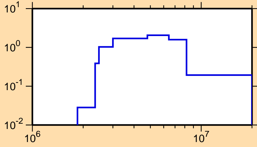
\sigma vs. E for ^{175}\text{Tm}(n,n\text{cont.})
