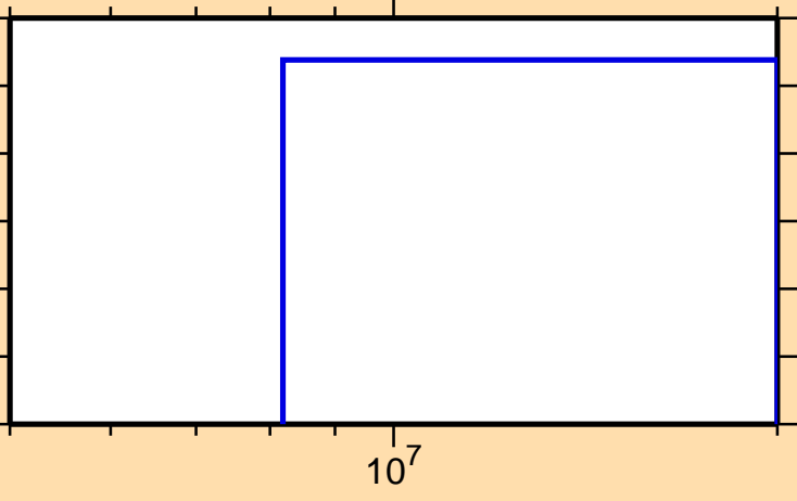
\sigma vs. E for ^{175}\text{Tm}(n,nt)
