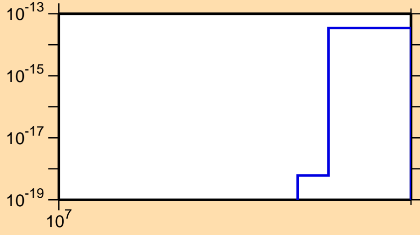
\sigma vs. E for ^{176}\text{Tm}(n,\text{He3})
