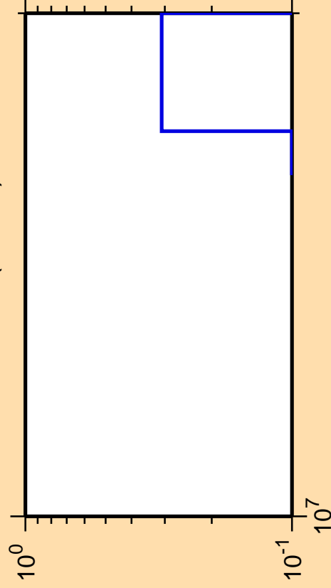
\Delta\sigma/\sigma vs. E for ^{176}\text{Tm}(n,\text{He3})
