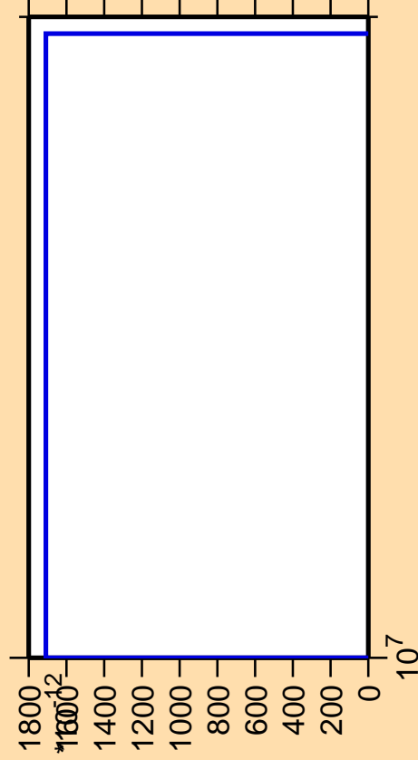
\Delta\sigma/\sigma vs. E for ^{176}\text{Tm} (mt 42)
