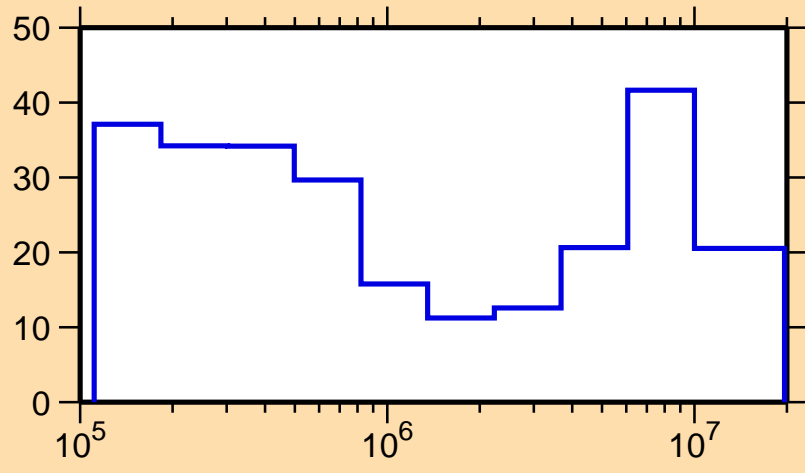
\Delta\sigma/\sigma vs. E for ^{176}\text{Tm}(n,\text{inel.})
