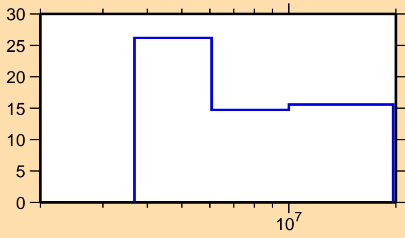
\Delta\sigma/\sigma vs. E for ^{176}\text{Tm}(n,2n)
