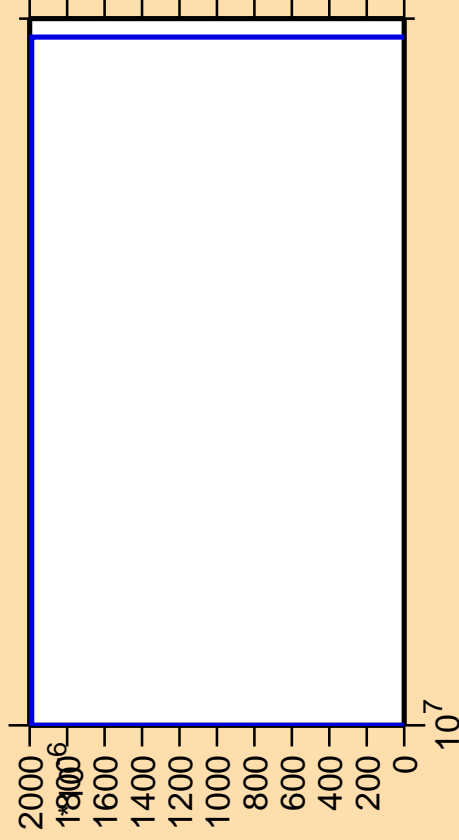
\Delta\sigma/\sigma vs. E for ^{176}\text{Tm}(n,\text{He}3)
