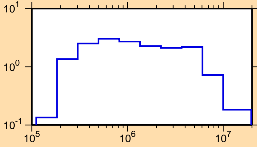
\sigma vs. E for ^{176}\text{Tm}(n,\text{inel.})
