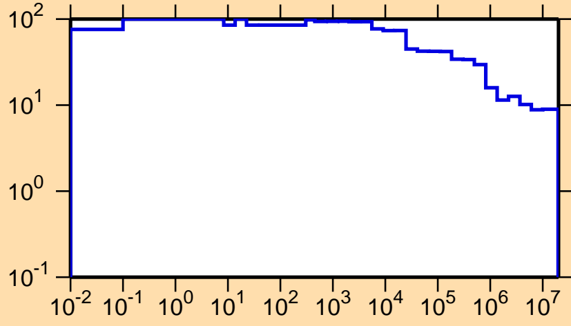
\Delta\sigma/\sigma vs. E for ^{176}\text{Tm}(n,\text{nonel.})
