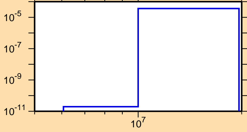
\sigma vs. E for ^{176}\text{Tm}(n,t)
