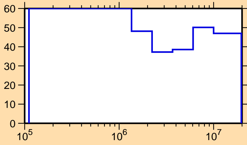
\Delta\sigma/\sigma vs. E for ^{176}\text{Tm}(n,n_1)
