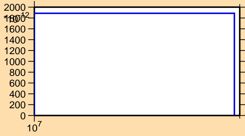
\sigma vs. E for ^{176}\text{Tm}(n,2n\alpha)
