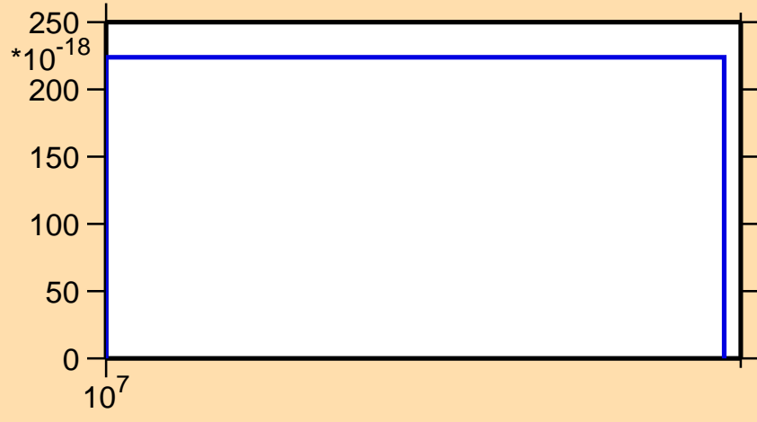
\sigma vs. E for ^{176}\text{Tm}(n,\text{He}3)
