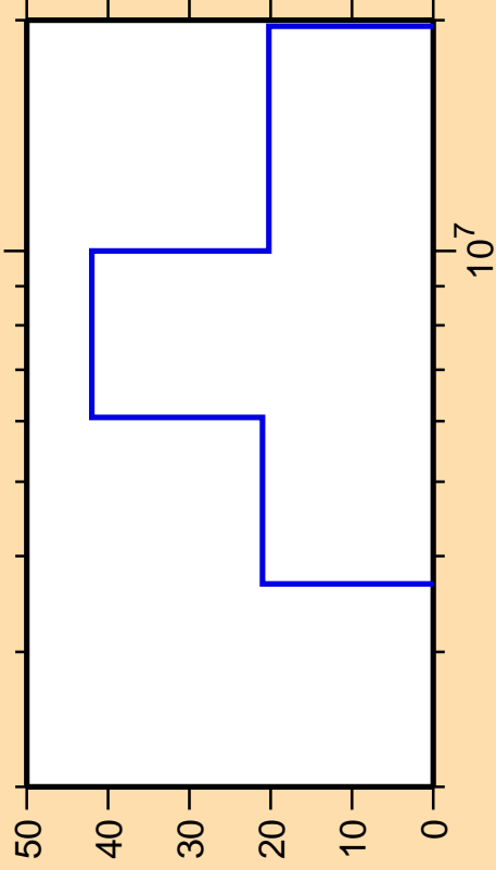
\Delta\sigma/\sigma vs. E for ^{176}\text{Tm}(n,n\text{cont.})
