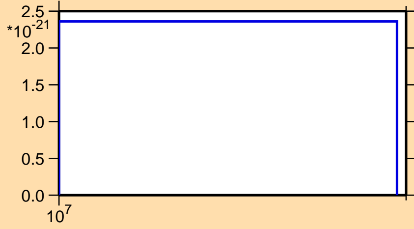
\sigma vs. E for ^{176}\text{Tm} (mt 42)
