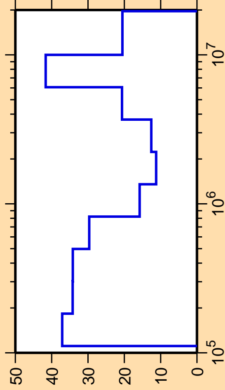
\Delta\sigma/\sigma vs. E for ^{176}\text{Tm}(n,\text{inel.})
