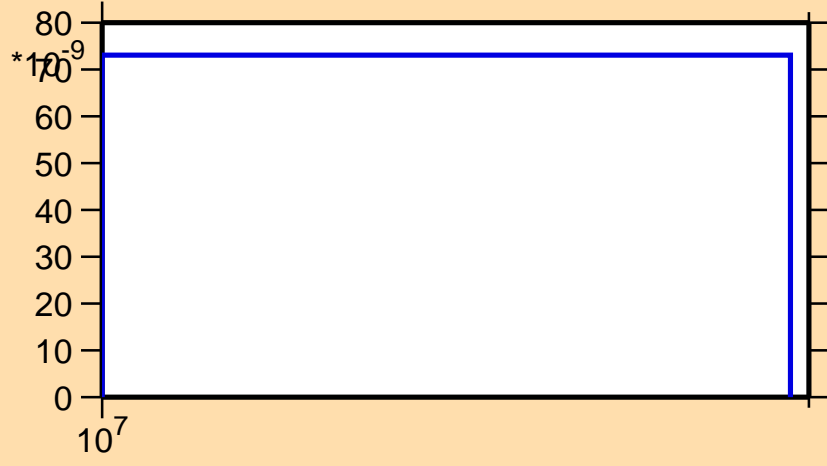
\sigma vs. E for ^{176}\text{Tm}(n,nt)
