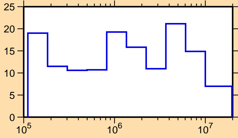
\Delta\sigma/\sigma vs. E for ^{176}\text{Tm}(n, el.)
