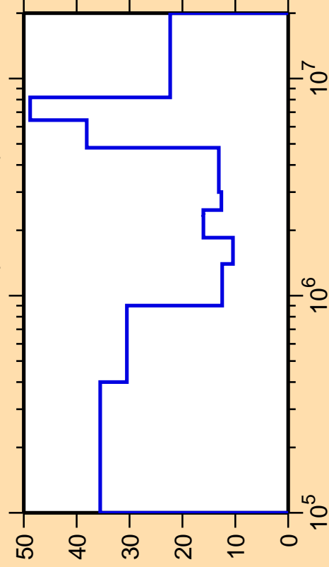
\Delta\sigma/\sigma vs. E for ^{176}\text{Tm}(n,ncont.)
