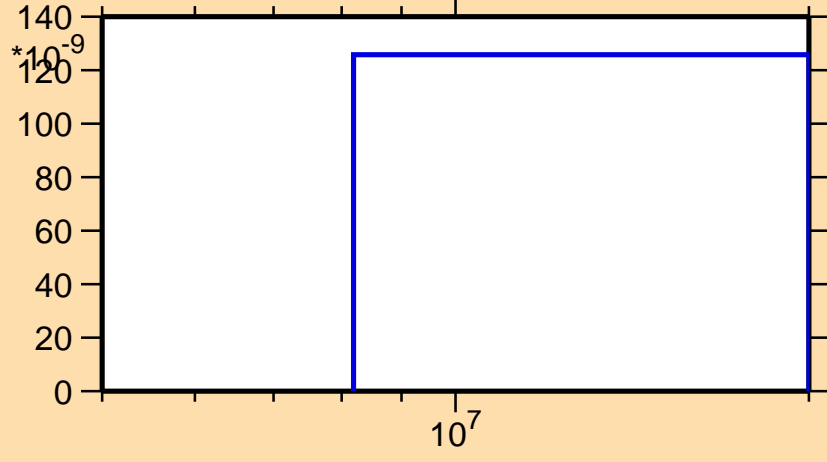
\sigma vs. E for ^{176}\text{Tm}(n,\text{nd})
