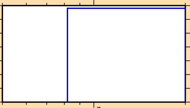
\sigma vs. E for ^{176}\text{Tm}(n,2np)
