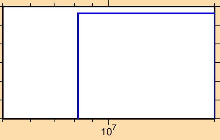
\sigma vs. E for ^{176}\text{Tm}(n,\text{He3})
