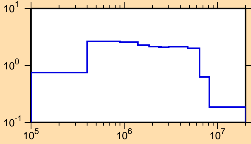
\sigma vs. E for ^{176}\text{Tm}(n,n\text{cont.})
