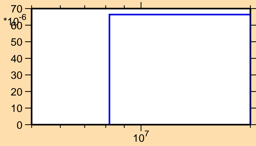
\sigma vs. E for ^{176}\text{Tm}(n,np)
