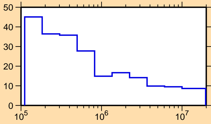
\Delta\sigma/\sigma vs. E for ^{177}\text{Tm}(n, nonel.)
