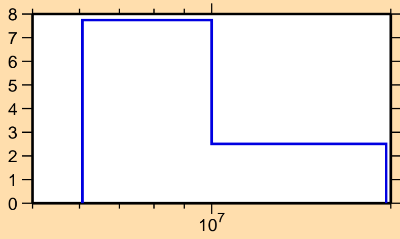
\Delta\sigma/\sigma vs. E for ^{177}\text{Tm}(n,\text{tot.})
