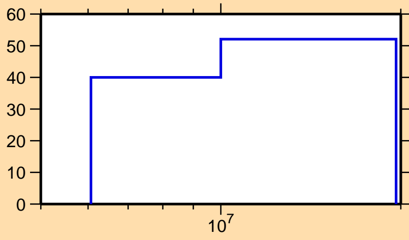
\Delta\sigma/\sigma vs. E for ^{177}\text{Tm}(n,ncont.)
