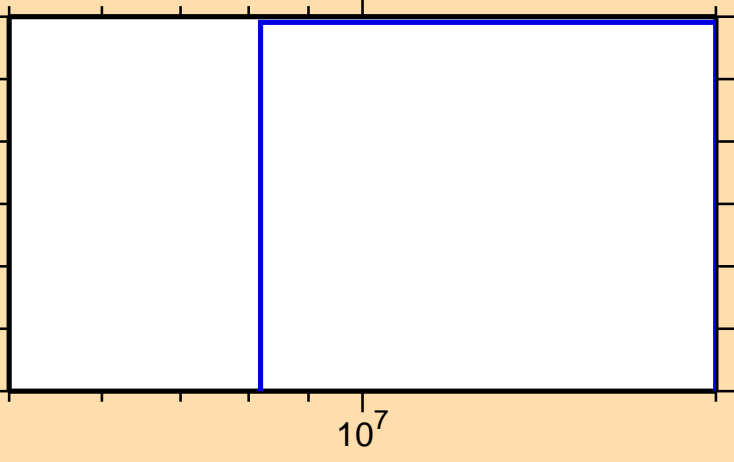
\sigma vs. E for ^{177}\text{Tm}(n,nd)
