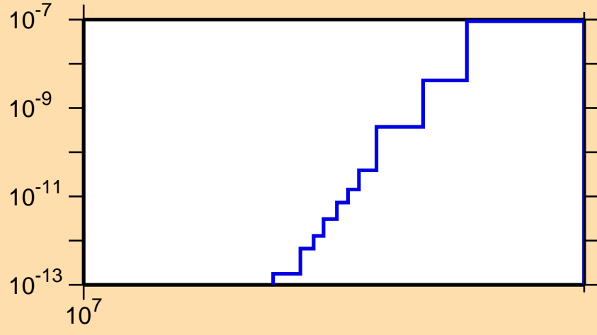
\sigma vs. E for ^{178}\text{Tm}(n,2n\alpha)
