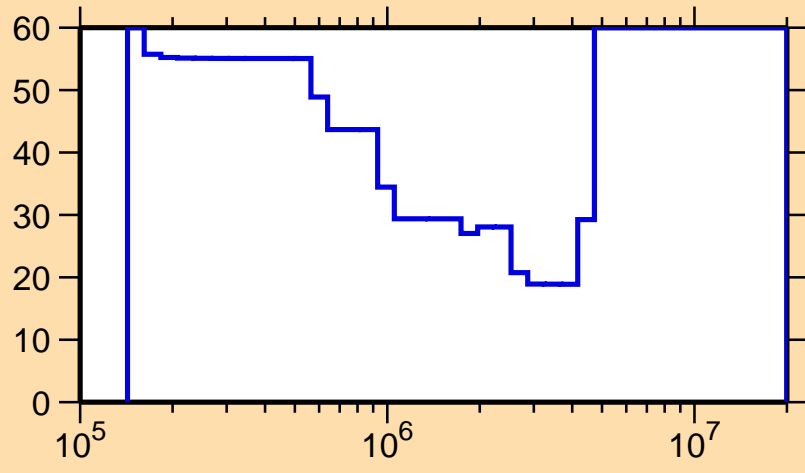
\Delta\sigma/\sigma vs. E for ^{178}\text{Tm}(n,n\text{cont.})
