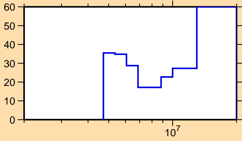
\Delta\sigma/\sigma vs. E for ^{178}\text{Tm}(n,2n)
