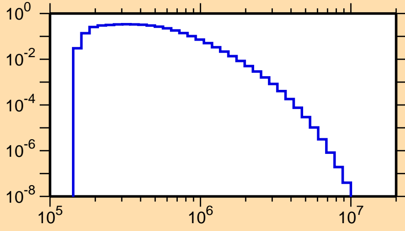
\sigma vs. E for ^{178}\text{Tm}(n,n_1)
