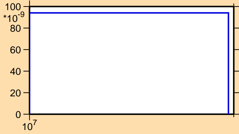
\sigma vs. E for ^{178}\text{Tm}(n,nt)
