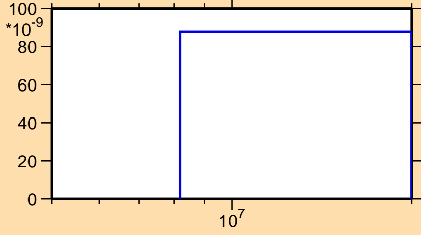
\sigma vs. E for ^{178}\text{Tm}(n,\text{nd})
