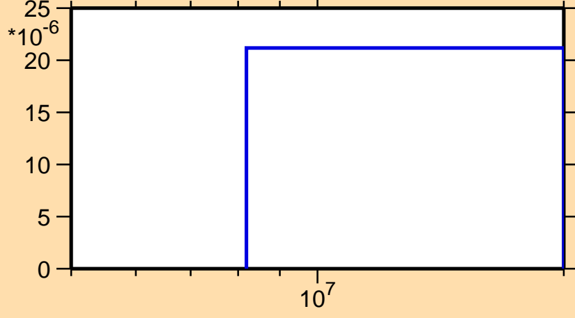
\sigma vs. E for ^{178}\text{Tm}(n,t)
