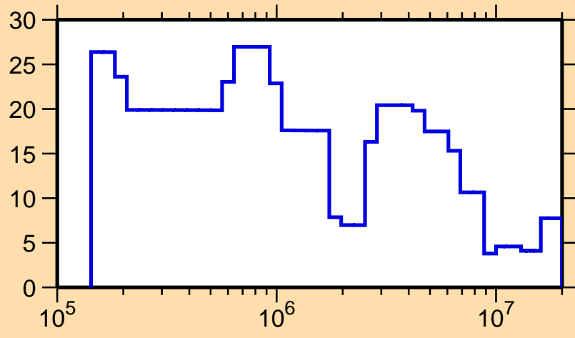
\Delta\sigma/\sigma vs. E for ^{179}\text{Tm}(n, tot.)
