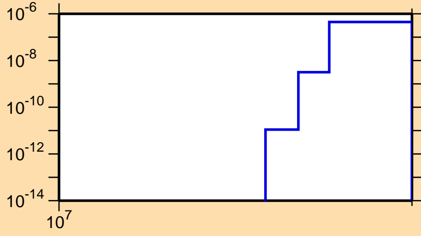
\sigma vs. E for ^{179}\text{Tm}(n,nd)
