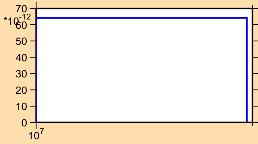
\sigma vs. E for ^{179}\text{Tm}(n,2np)
