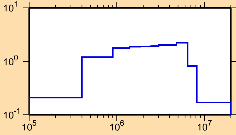
\sigma vs. E for ^{179}\text{Tm}(n,n\text{cont.})
