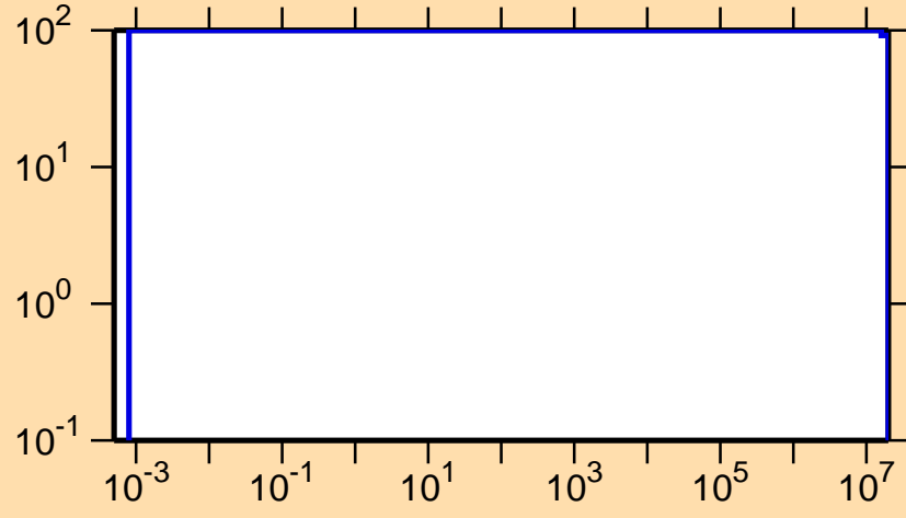
\Delta\sigma/\sigma vs. E for ^{227}\text{U}(n,p)
