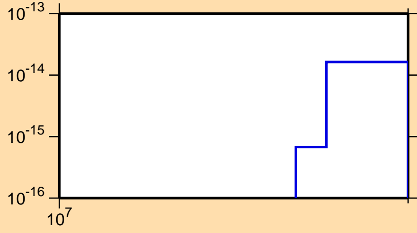
\sigma vs. E for ^{227}\text{U}(n,\text{pt})
