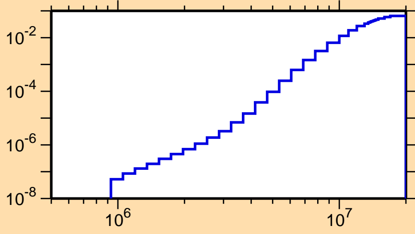
\sigma vs. E for ^{227}\text{U}(n,p)
