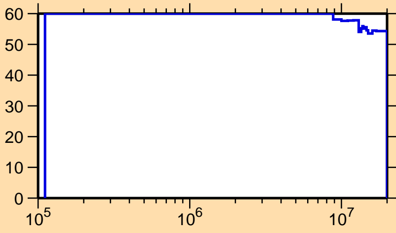
\Delta\sigma/\sigma vs. E for ^{227}\text{U}(n,n_1)
