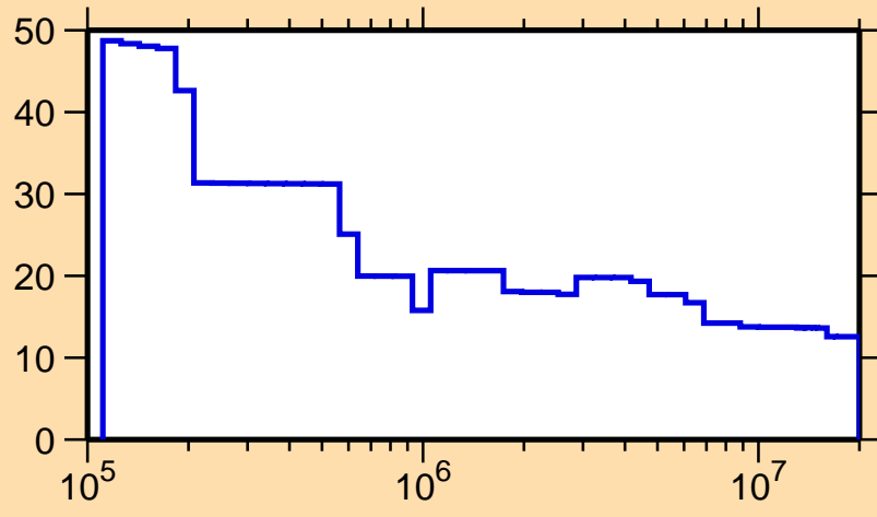
\Delta\sigma/\sigma vs. E for ^{227}\text{U}(n, nonel.)
