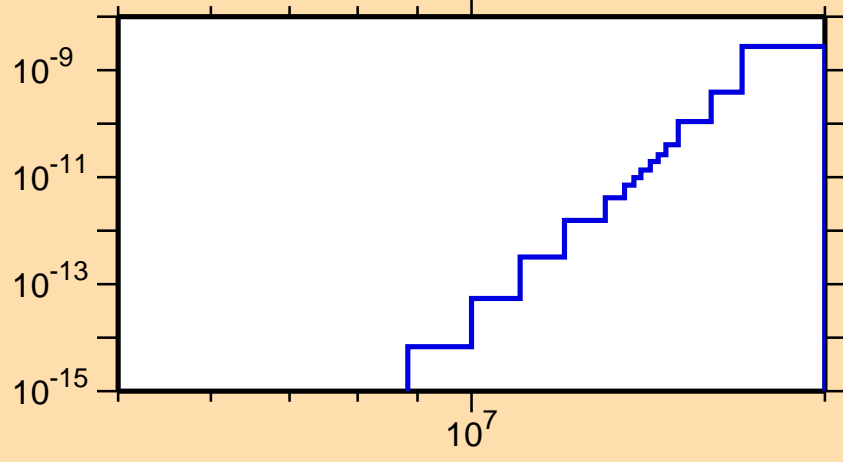
\sigma vs. E for ^{227}\text{U}(n,\text{He3})
