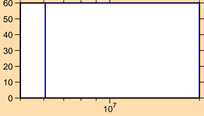
\Delta\sigma/\sigma vs. E for ^{227}\text{U}(n,2n)
