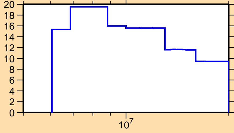
\Delta\sigma/\sigma vs. E for ^{227}\text{U}(n,\text{tot.})
