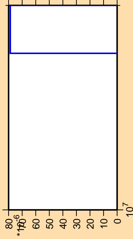
\Delta\sigma/\sigma vs. E for ^{227}\text{U} (mt 42)
