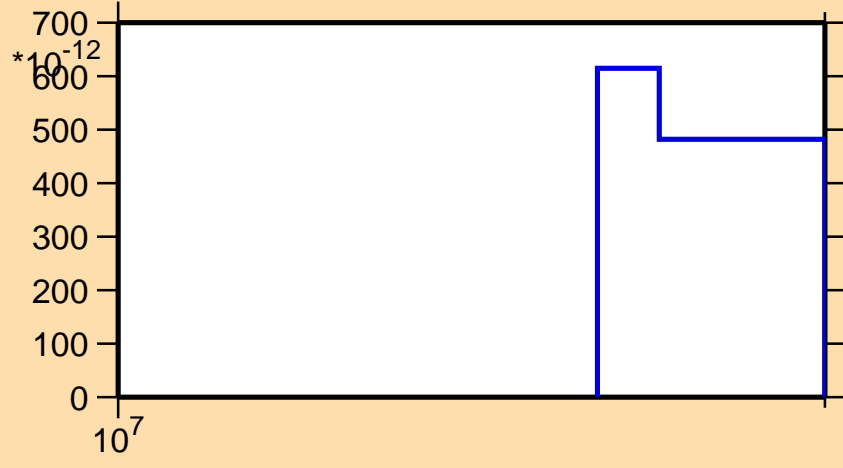
\sigma vs. E for ^{227}\text{U}(\text{mt117})
