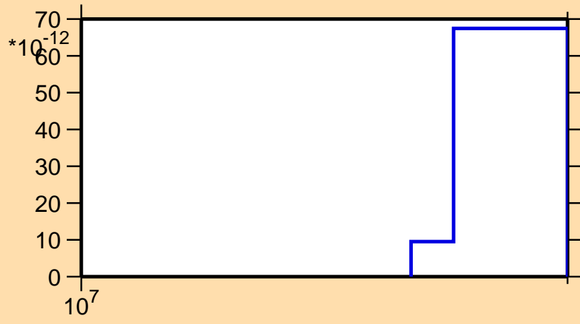
\sigma vs. E for ^{227}\text{U} (mt 34)
