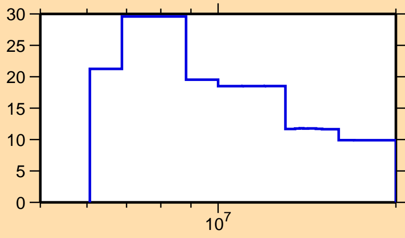
\Delta\sigma/\sigma vs. E for ^{227}\text{U}(n,\text{el.})
