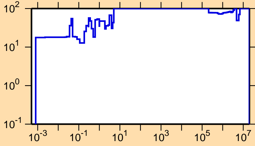
\Delta\sigma/\sigma vs. E for ^{227}\text{U}(n,\gamma)
