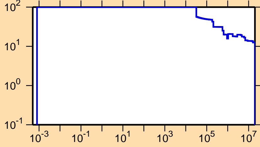
\Delta\sigma/\sigma vs. E for ^{227}\text{U}(n,\text{nonel.})
