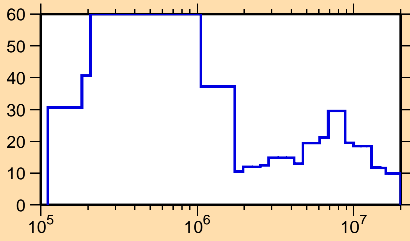
\Delta\sigma/\sigma vs. E for ^{227}\text{U}(n, el.)
