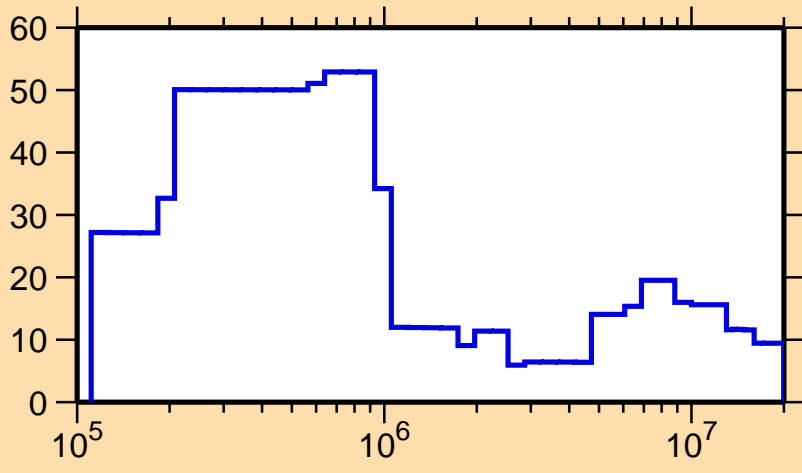
\Delta\sigma/\sigma vs. E for ^{227}\text{U}(n,\text{tot.})
