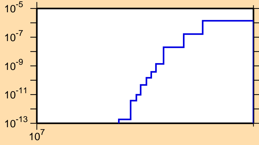
\sigma vs. E for ^{227}\text{U}(n,2np)
