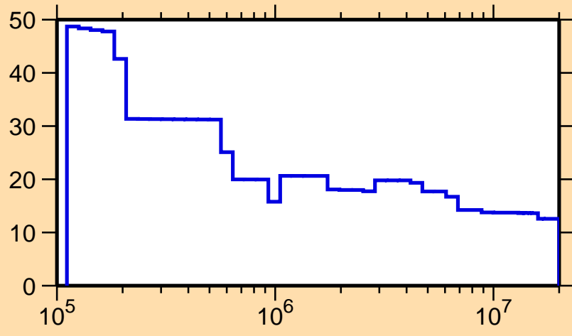
\Delta\sigma/\sigma vs. E for ^{227}\text{U}(n,\text{nonel.})
