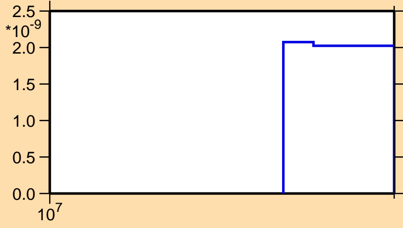
\sigma vs. E for ^{227}\text{U} (mt 45)
