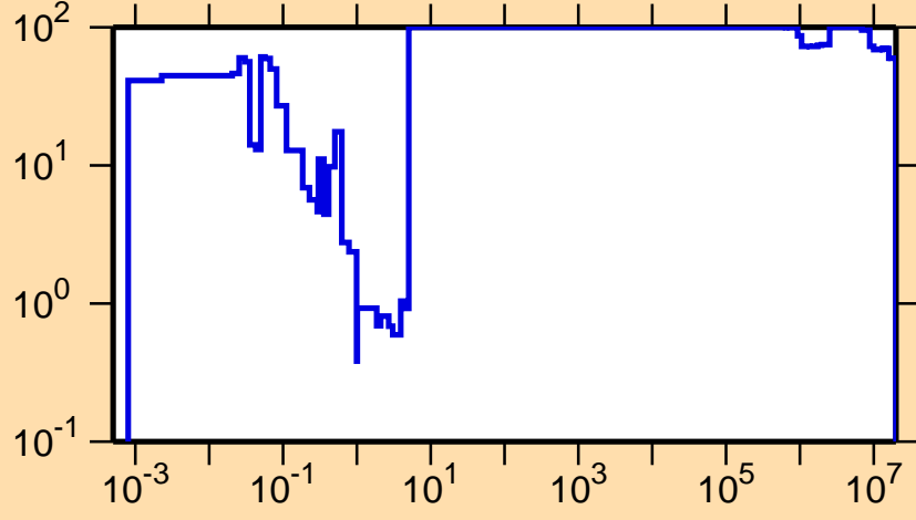
\Delta\sigma/\sigma vs. E for ^{227}\text{U}(n,f)
