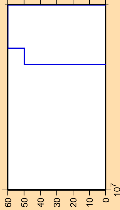
\Delta\sigma/\sigma vs. E for ^{227}\text{U} (mt 34)
