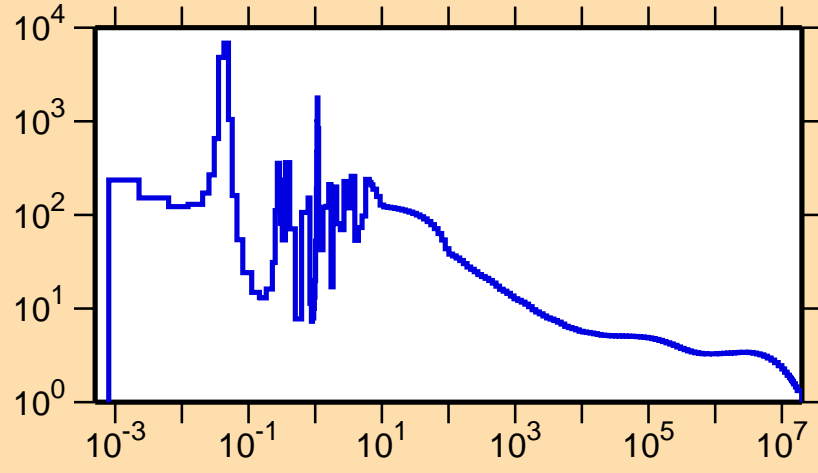
\sigma vs. E for ^{227}\text{U}(n,f)
