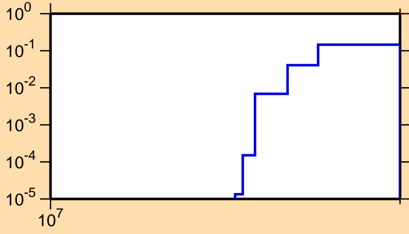
\sigma vs. E for ^{227}\text{U}(n,3n)
