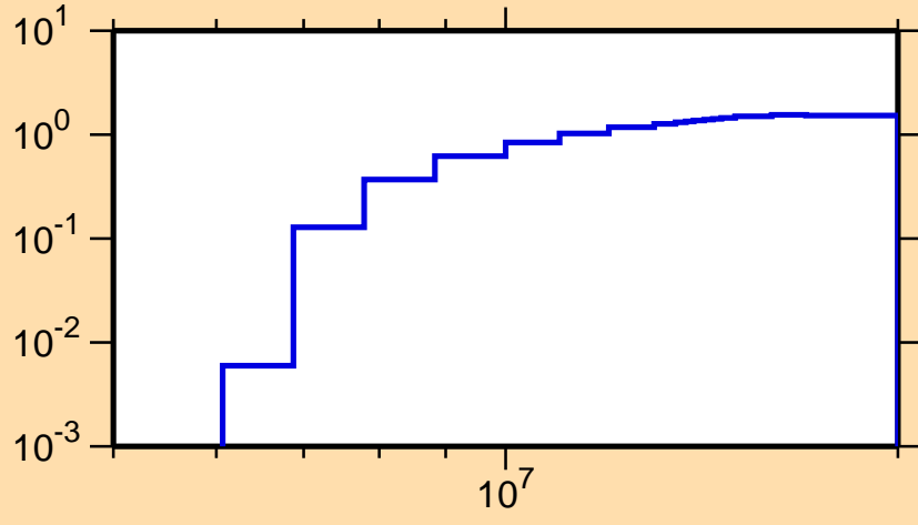
\sigma vs. E for ^{227}\text{U}(n,2n)
