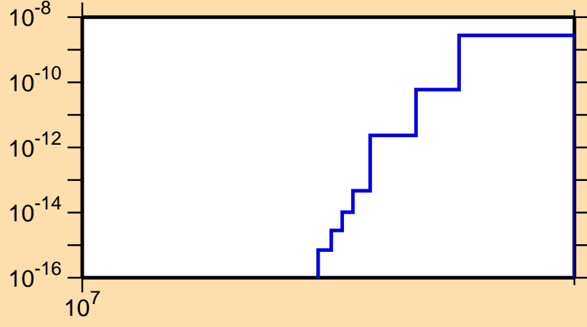
\sigma vs. E for ^{227}\text{U}(n,nt)
