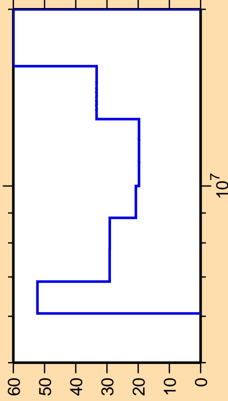
\Delta\sigma/\sigma vs. E for ^{227}\text{U}(n,\alpha)
