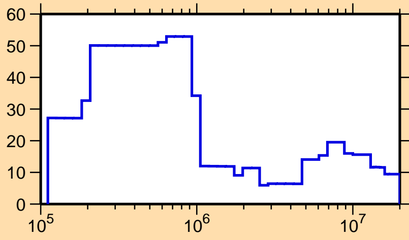
\Delta\sigma/\sigma vs. E for ^{227}\text{U}(n, tot.)
