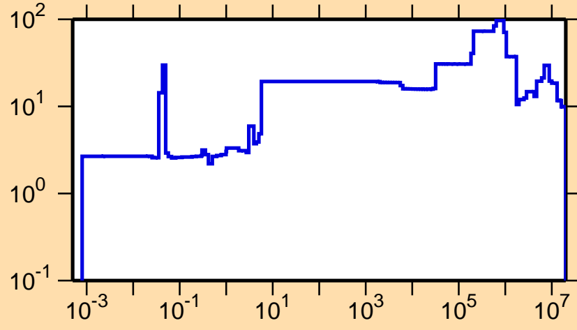
\Delta\sigma/\sigma vs. E for ^{227}\text{U}(n,el.)
