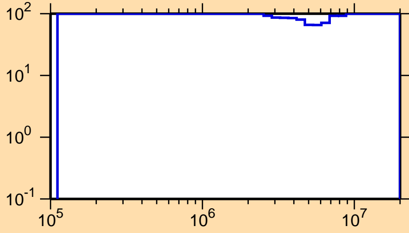
\Delta\sigma/\sigma vs. E for ^{227}\text{U}(n,n\text{cont.})
