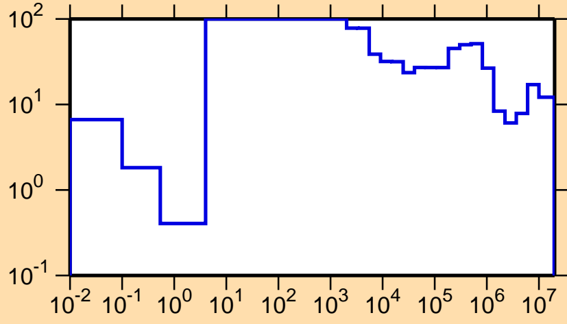
\Delta\sigma/\sigma vs. E for ^{227}\text{U}(n,tot.)
