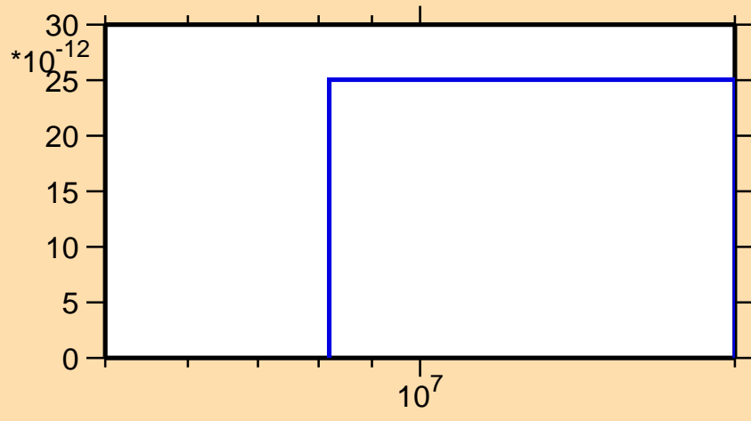
\sigma vs. E for ^{227}\text{U}(n,nt)
