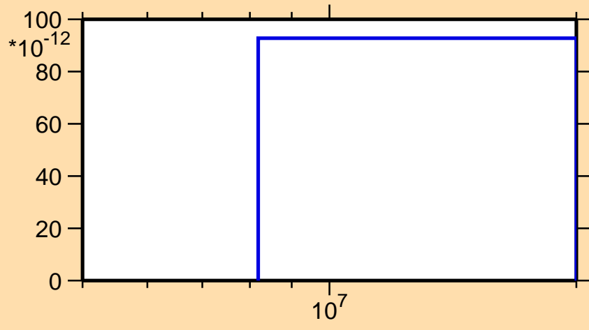
\sigma vs. E for ^{227}\text{U}(\text{mt117})
