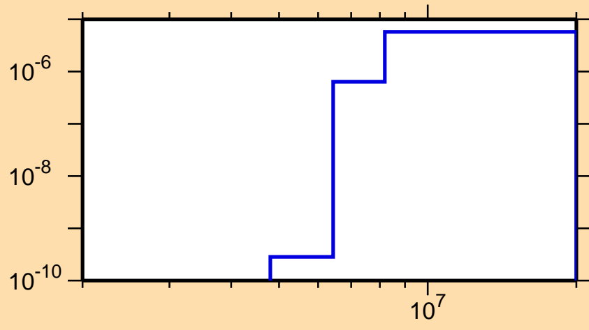
\sigma vs. E for ^{227}\text{U}(n,2n\alpha)
