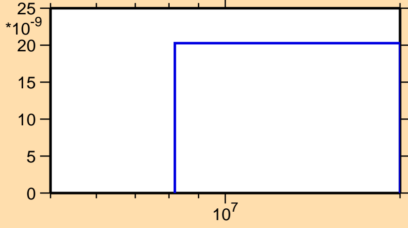
\sigma vs. E for ^{227}\text{U}(n,2np)
