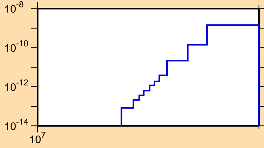
\sigma vs. E for ^{228}\text{U}(n,\text{He3})
