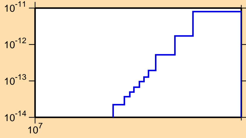
\sigma vs. E for ^{228}\text{U}(n,p\alpha)
