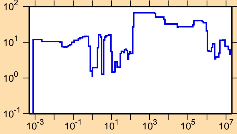
\Delta\sigma/\sigma vs. E for ^{228}\text{U}(n,tot.)
