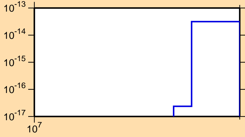
\sigma vs. E for ^{228}\text{U} (mt 34)
