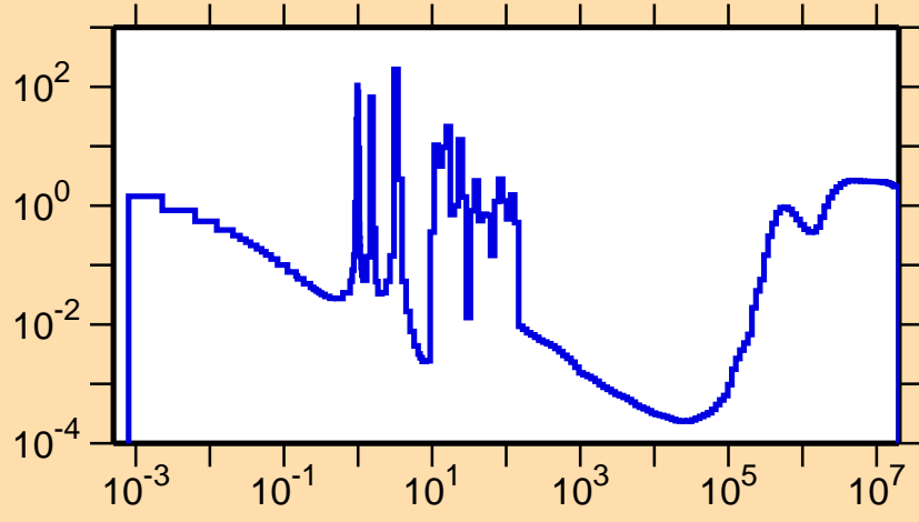
\sigma vs. E for ^{228}\text{U}(n,f)
