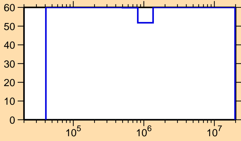
\Delta\sigma/\sigma vs. E for ^{228}\text{U}(n,inel.)
