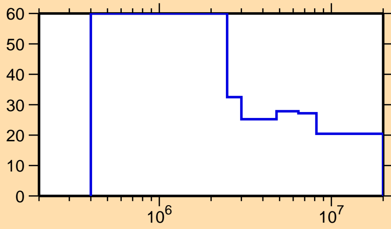
\Delta\sigma/\sigma vs. E for ^{228}\text{U}(n,n_1)
