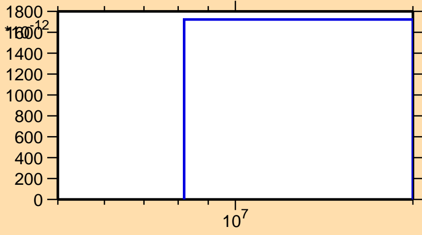
\sigma vs. E for ^{228}\text{U}(n,\text{nd})
