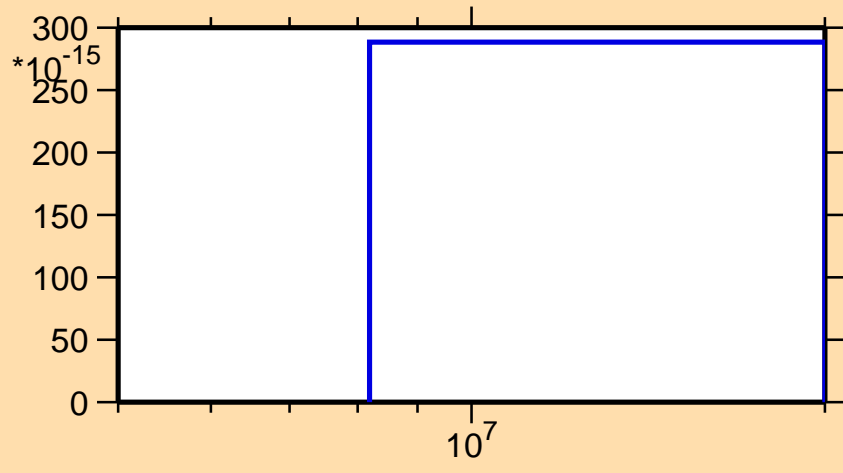
\sigma vs. E for ^{228}\text{U} (mt 45)
