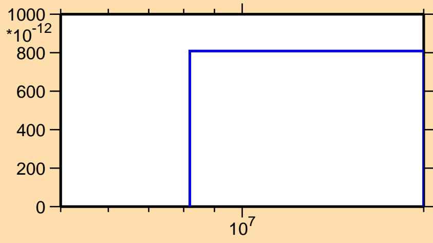
\sigma vs. E for ^{228}\text{U}(n,2np)
