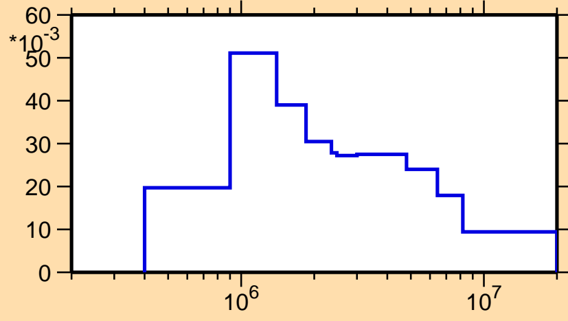
\sigma vs. E for ^{228}\text{U}(n,n_3)
