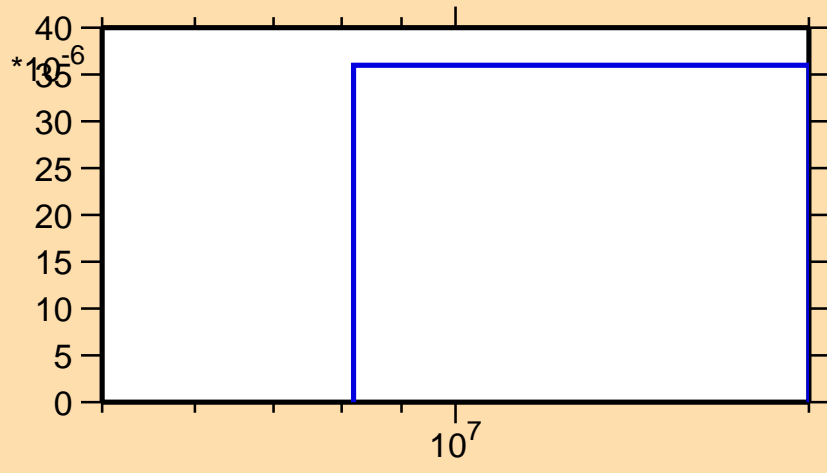
\sigma vs. E for ^{228}\text{U}(n,t)
