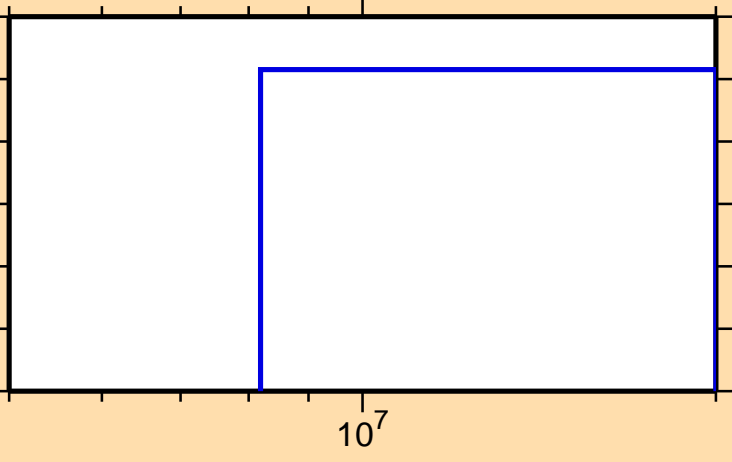
\sigma vs. E for ^{228}\text{U} (mt 34)
