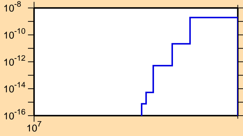
\sigma vs. E for ^{229}\text{U}(n,nt)
