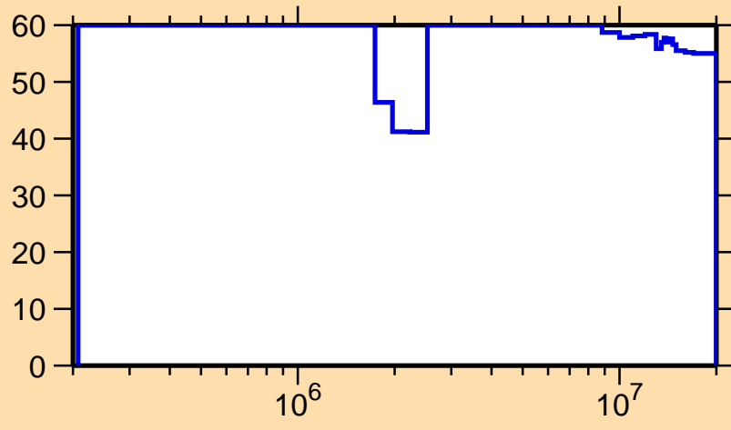
\Delta\sigma/\sigma vs. E for ^{229}\text{U}(n, inel.)
