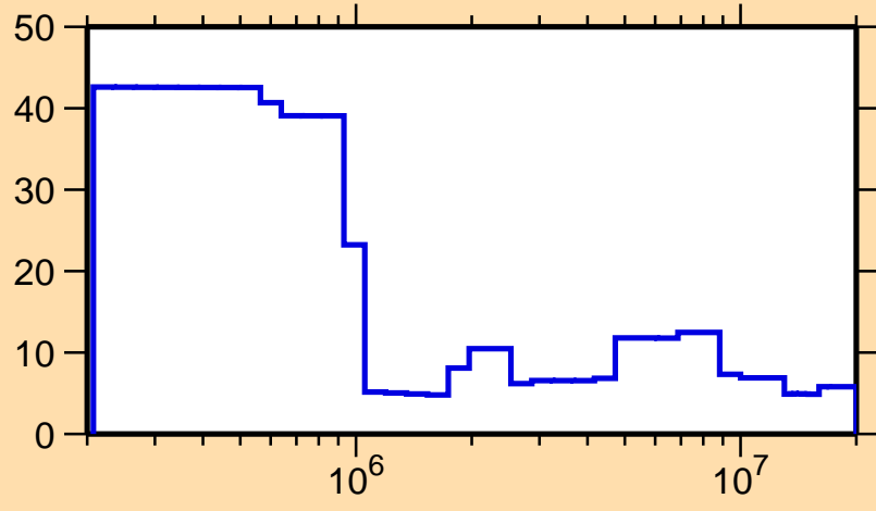
\Delta\sigma/\sigma vs. E for ^{229}\text{U}(n, tot.)
