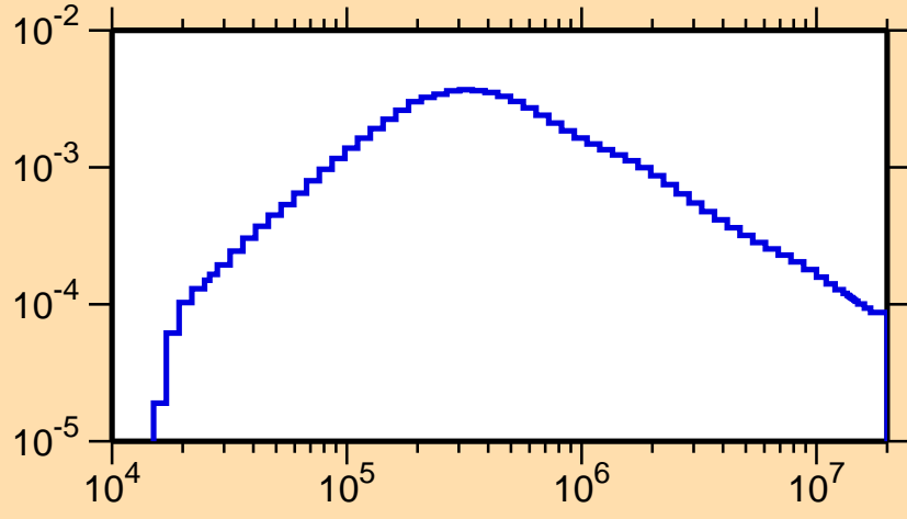
\sigma vs. E for ^{229}\text{U}(n,n_1)
