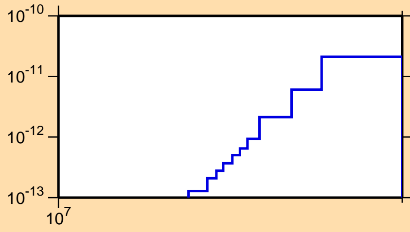
\sigma vs. E for ^{229}\text{U}(n,p\alpha)
