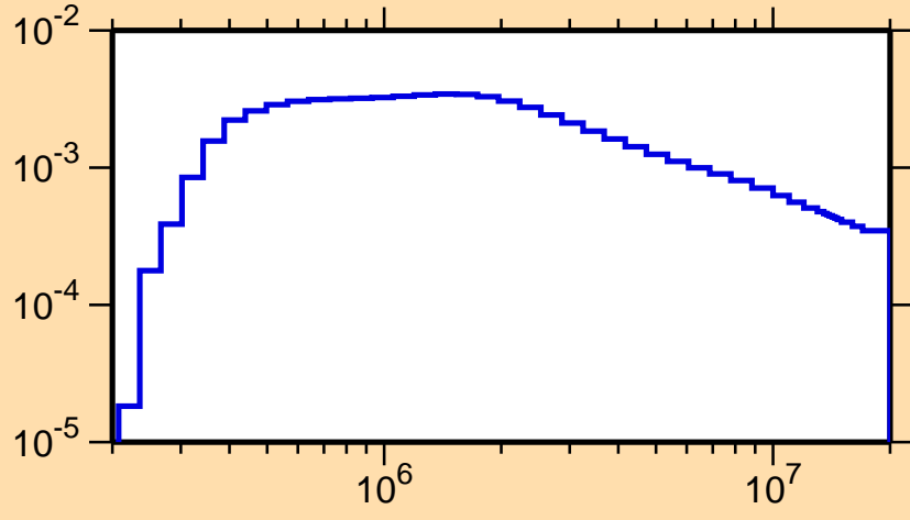
\sigma vs. E for ^{229}\text{U}(n,n_2)
