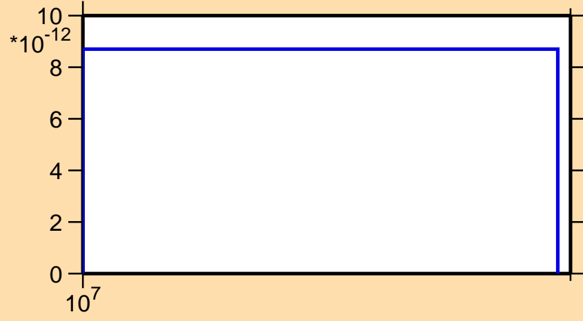
\sigma vs. E for ^{229}\text{U}(n,nd)
