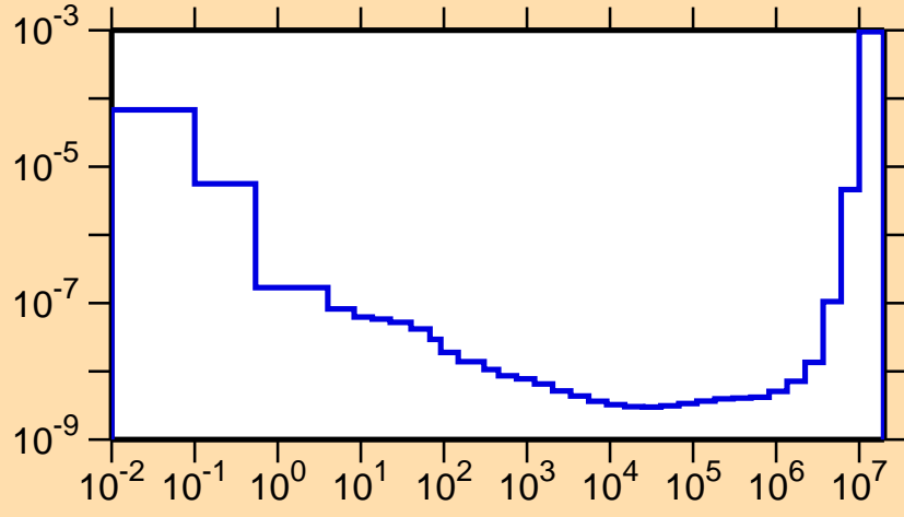
\sigma vs. E for ^{229}\text{U}(n,\alpha)
