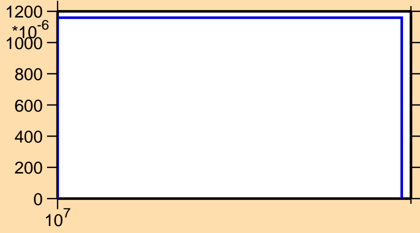
\sigma vs. E for ^{229}\text{U}(n,3n)
