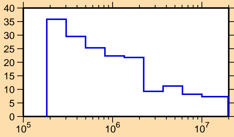
\Delta\sigma/\sigma vs. E for ^{229}\text{U}(n, nonel.)
