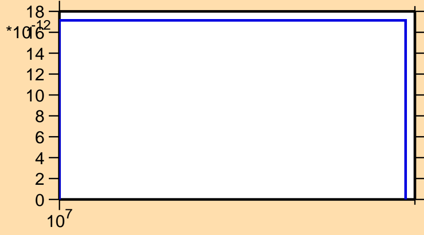
\sigma vs. E for ^{229}\text{U}(n,nt)
