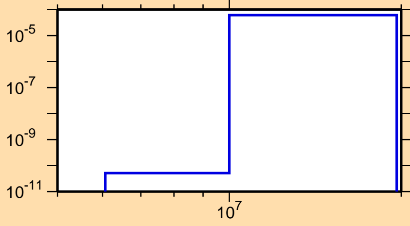
\sigma vs. E for ^{229}\text{U}(n,t)
