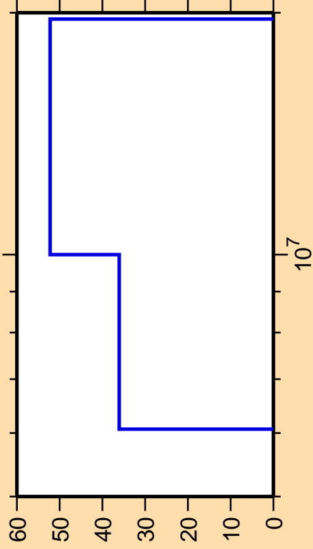
\Delta\sigma/\sigma vs. E for ^{229}\text{U}(n,t)
