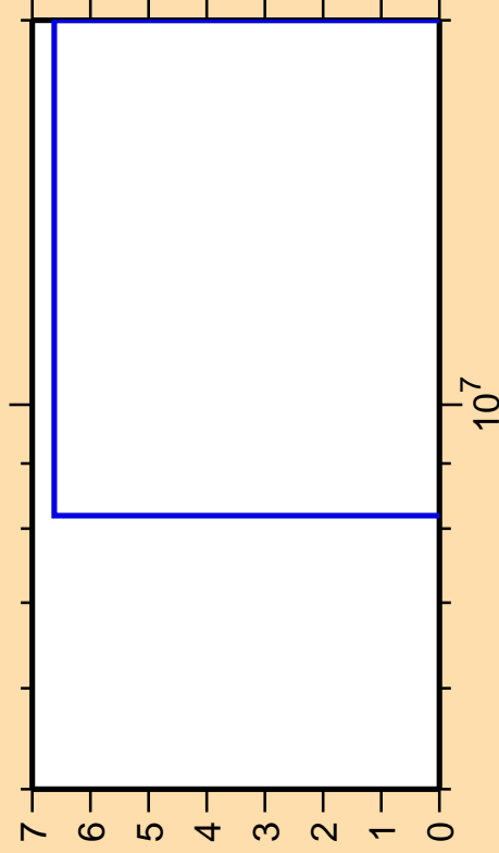
\Delta\sigma/\sigma vs. E for ^{229}\text{U}(n,p\alpha)
