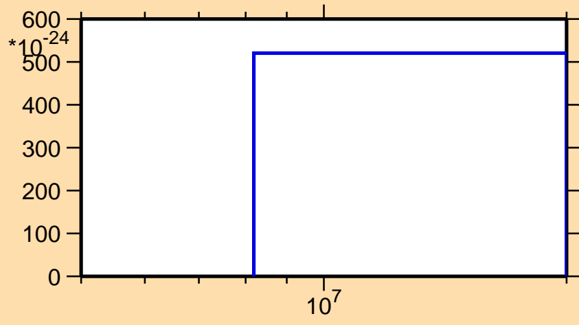
\sigma vs. E for ^{229}\text{U} (mt 42)
