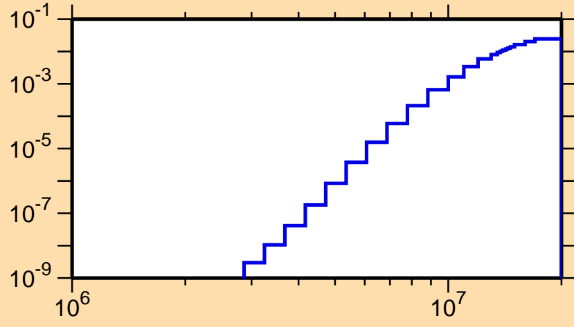
\sigma vs. E for ^{231}\text{U}(n,p)
