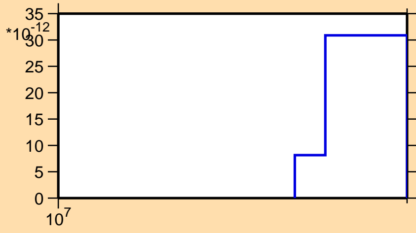
\sigma vs. E for ^{231}\text{U}(n,p\alpha)
