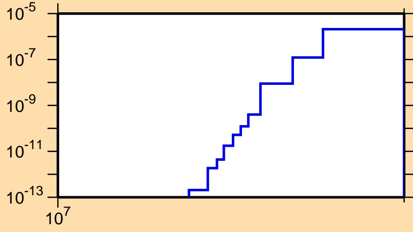
\sigma vs. E for ^{231}\text{U}(n,nd)
