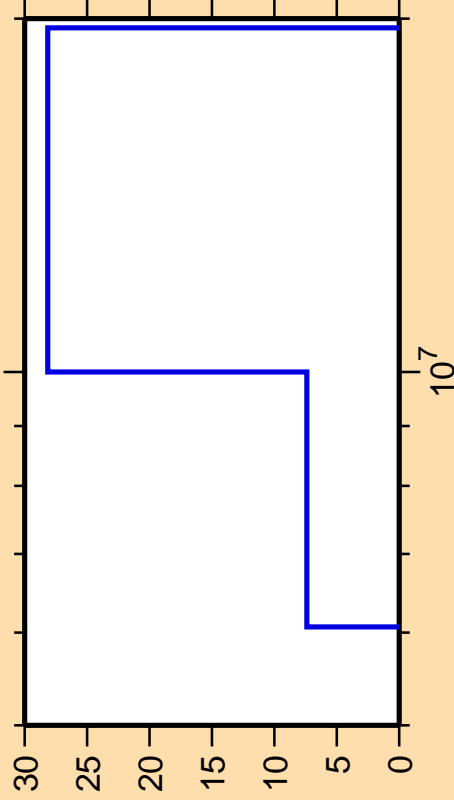
\Delta\sigma/\sigma vs. E for ^{231}\text{U}(n,t)
