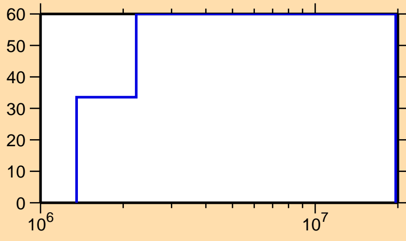
\Delta\sigma/\sigma vs. E for ^{231}\text{U}(n,p)
