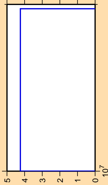
\Delta\sigma/\sigma vs. E for ^{231}\text{U}(n,p\alpha)
