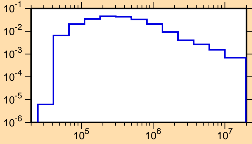
\sigma vs. E for ^{231}\text{U}(n,n_1)
